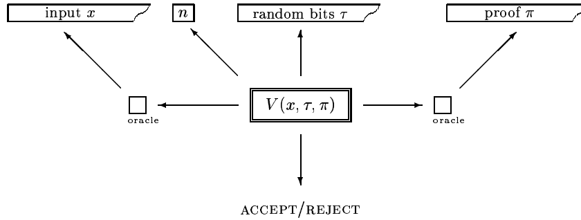
Figure 4: A verifier for probabilistically checkable languages
