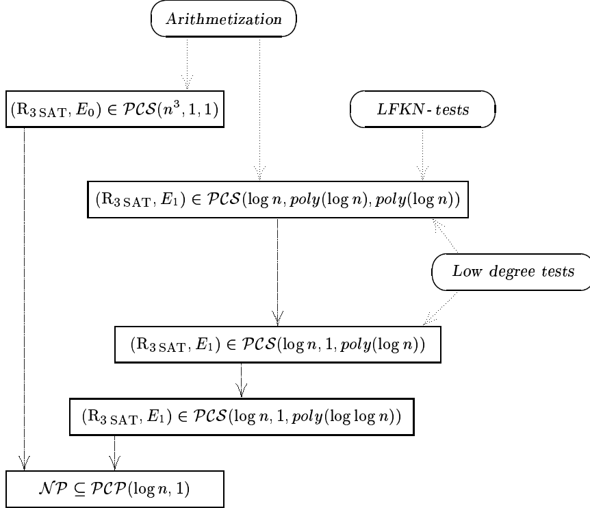
Figure 2: Structure of the proof of Theorem 2.2
