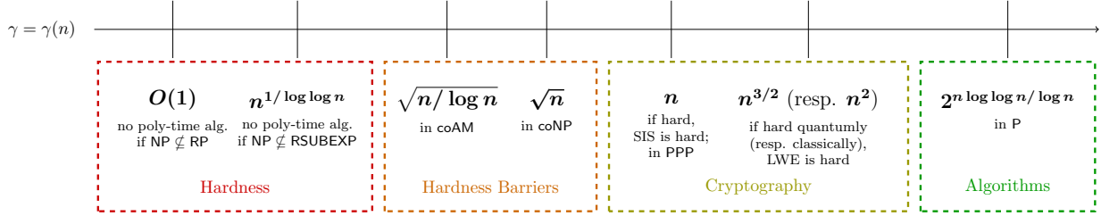
Figure 3: A summary of the complexity of \gamma -GapSVP on lattices of dimension n for approximation factors \gamma = \gamma(n) , with some constants and lower-order terms omitted for clarity. The figure shows polynomial-time algorithms, worst-case to average-case reductions, and protocols, as well as hardness results ruling out polynomial-time algorithms.
