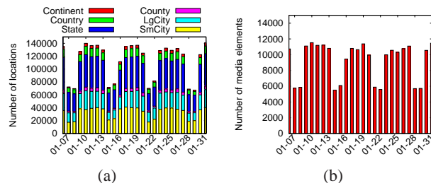
Figure 9: Different types of content found by NewsStand in articles, including (a) number and types of locations, and (b) amount of multimedia (images and videos).
