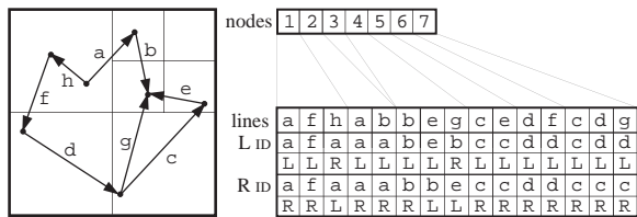
Figure 8: Polygon assignments after the first round of leaf node merging.
