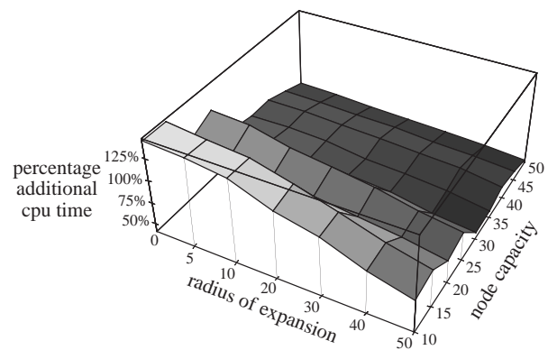
Figure 17: Percentage of additional execution time required by the leaf node intersection determination phase of the bottom-up R-tree spatial join algorithm relative to the top-down algorithm.
