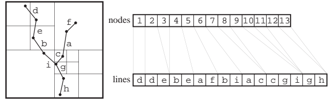
Figure 5: Result of the bucket PMR quadtree build process.
