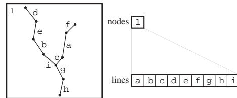
Figure 1: Initial bucket PMR quadtree processor assignments.
