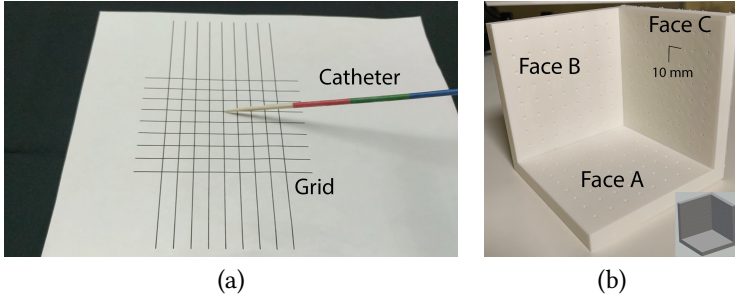
Fig. 9. Setup for testing (a) the tracking accuracy over a 2D grid, and (b) tracking accuracy over a 3D grid with the 3D CAD model in the lower right
