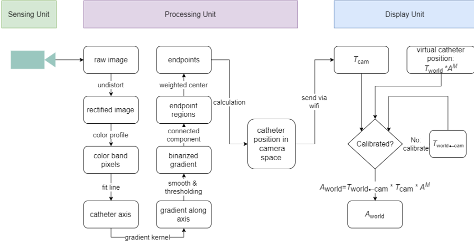
Fig. 3. The workflow of the system
