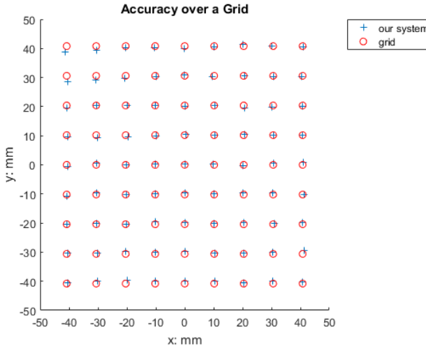
Fig. 10. The accuracy of our catheter tracking approach over the 2D grid. The red circles indicate the grid intersection. The blue crosses indicate the computed catheter tip position.
