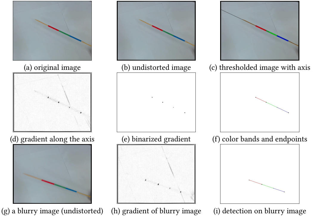
Fig. 8. Detecting endpoints. (g), (h) and (i) show detecting endpoints in an image where the catheter is blurry because of movement. Our algorithm is able to handle this case.
