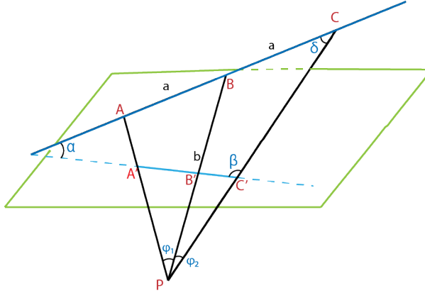
Fig. 6. We need to find the angle \alpha between the catheter and its image. Let A , B , and C be three endpoints of two consecutive color bands. The color bands are of equal length a . P is the center of projection in the pinhole camera model. The distance between B and P is b
