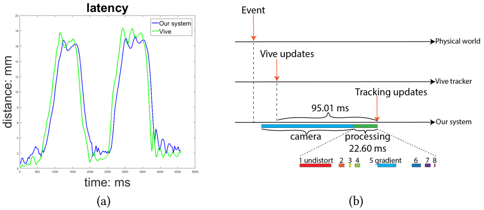
Fig. 11. The latency of our system compared to an HTC Vive tracker (a) and the various components of our system's latency in image capture and processing (b).
