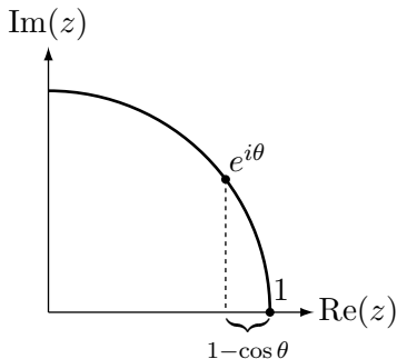
Figure 1: The classical gap, 1 - \lambda = 1 - \cos \theta , appears on the real axis. The quantum phase gap, \theta = \arccos \lambda , is quadratically larger, since \cos \theta \geq 1 - \theta^2/2 , i.e., \arccos \lambda \geq \sqrt{2(1 - \lambda)} .
