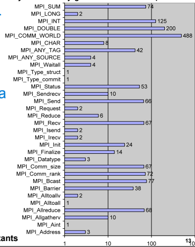
MPI keywords in Conjugate Gradient in C/C++ (15 students)
