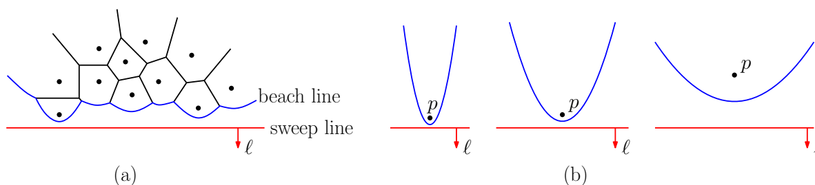
Fig. 5: The beach line. Notice that only the portion of the Voronoi diagram that lies above the beach line is computed. The sweep-line status maintains the intersection of the Voronoi diagram with the beach line.
