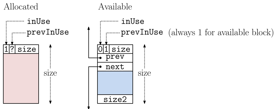
Fig. 118: Block structure for dynamic storage allocation.
