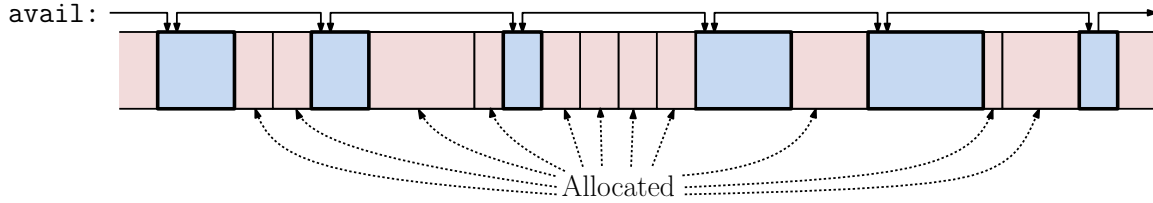
Fig. 117: Dynamic memory allocation block structure.
