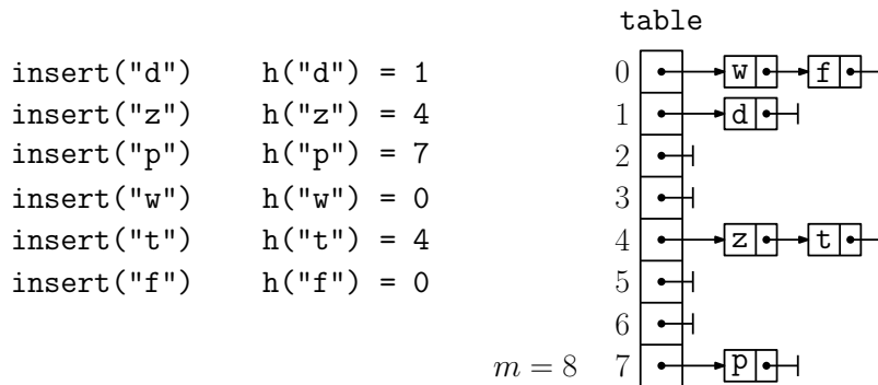
Fig. 94: Collision resolution by separate chaining.
