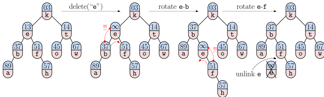
Fig. 56: Treap deletion.
