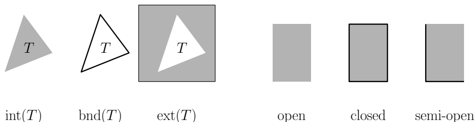
Fig. 135: Topological notation.
