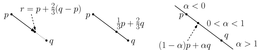
Fig. 137: Affine combinations.
