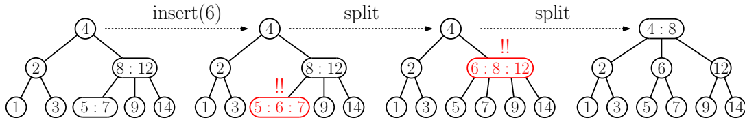
Fig. 42: 2-3 tree insertion involving two splits.
