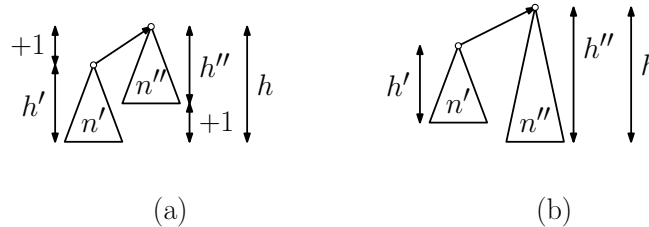
Fig. 17: Proof that n \geq 2^h .
