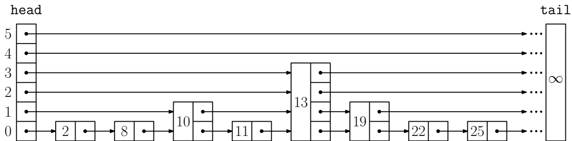
Fig. 59: A (randomized) skip list.
