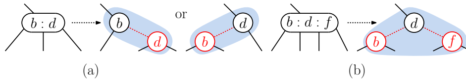
Fig. 47: Color combinations allowed by the red-black tree rules.
