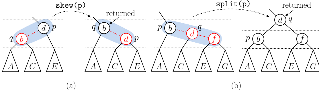
Fig. 49: AA restructuring operations (a) skew and (b) split . (Afterwards q may be red or black.)
