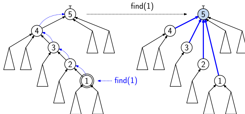
Fig. 18: Find using path compression.
