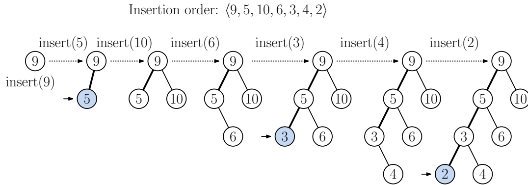
Fig. 31: Length of the leftmost chain.
