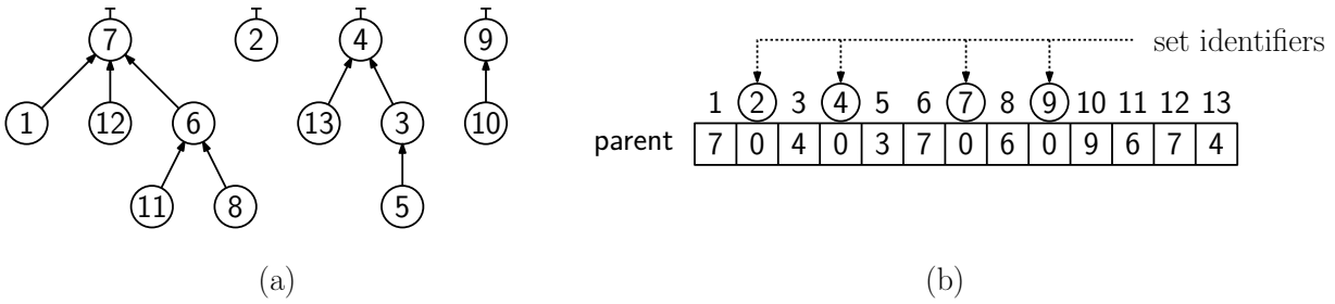
Fig. 14: (a) Partition stored as a forest of inverted trees and (b) array-based representation.
