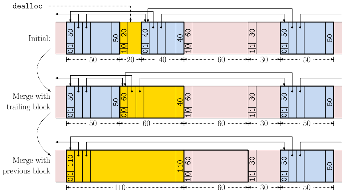
Fig. 120: An example of block deallocation and merging.
