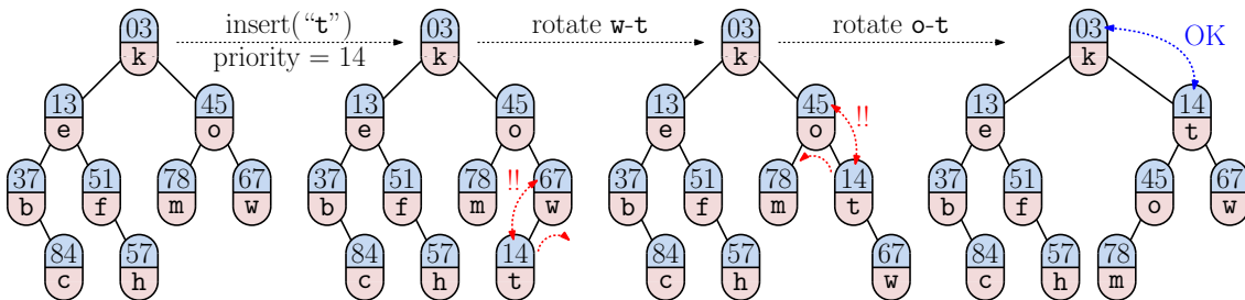
Fig. 55: Treap insertion.
