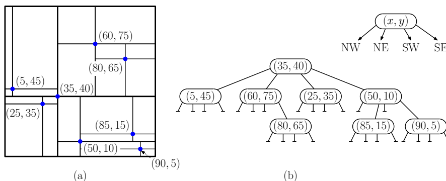
Fig. 72: Point quadtree.
