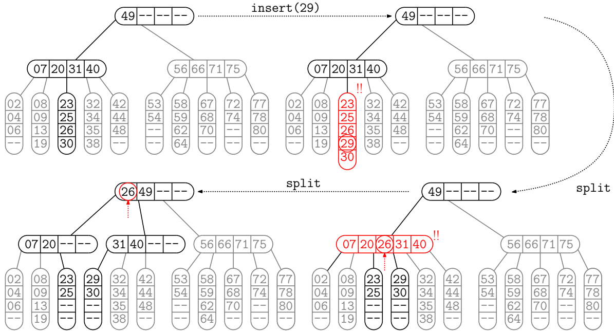
Fig. 105: Insertion of key 29 (order m = 5 ). It is inserted into the leaf node (23, 25, ...) which splits, causing the middle key 26 to be promoted to the parent, which also splits, causing the middle key 26 to be promoted to the root.
