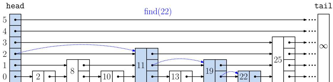
Fig. 58: Searching the ideal skip list.
