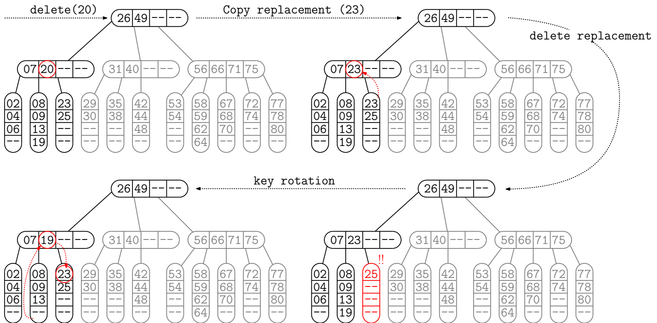
Fig. 106: Deletion of key 20 (order m = 5 ). Since 20 is not a leaf, we find the replacement 23 (inorder successor) and copy it there. We then delete 23 from its leaf, which underflows. The sibling rotates the key 19 to the parent and the parent gives up its key 23.
