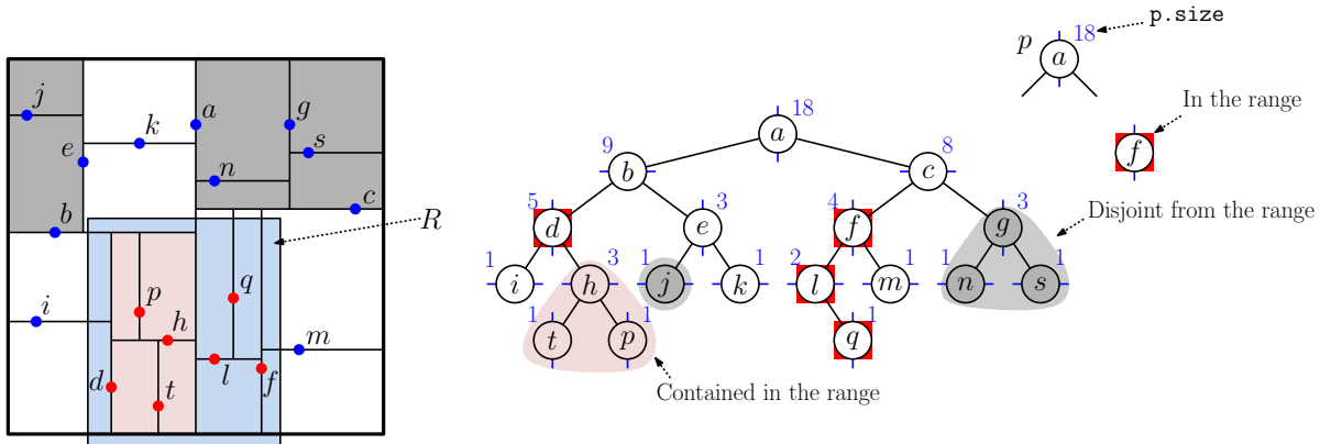
Fig. 82: Range search in kd-trees. The subtree rooted at h is counted entirely. The subtrees rooted at j and g are excluded entirely. The other points are checked individually.
