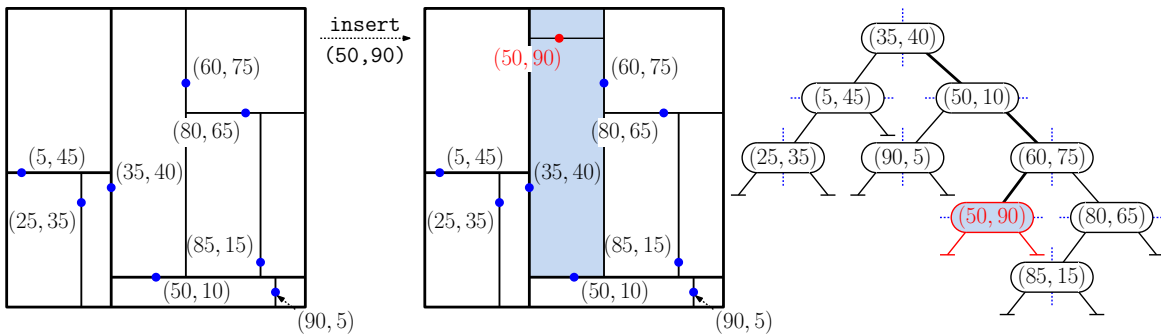
Fig. 74: Inserting (50, 90) into the point kd-tree of Fig. 73.
