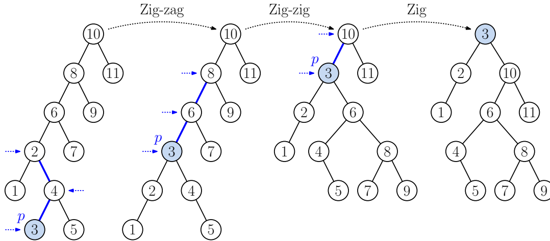
Fig. 67: The full splay operation on p .
