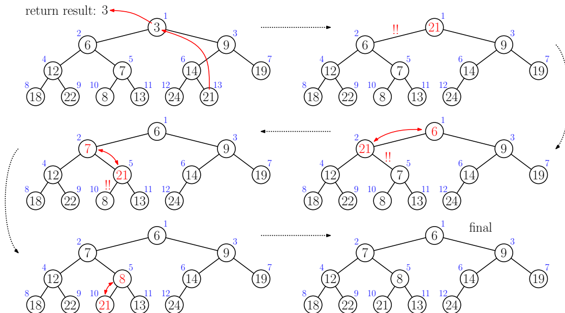
Fig. 22: Example of extract-min. We save the root element (3) as the final result, and copy the last element (21) into the root and decrement n . We then repeatedly sift it down by swapping it with the smaller of its two children until either reaching the leaf level or until both of its children are at least as large.
