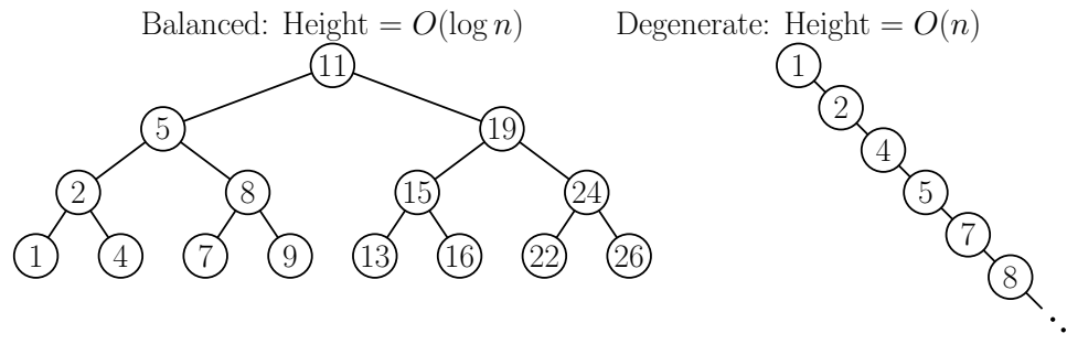
Fig. 27: Balanced and degenerate binary trees.
