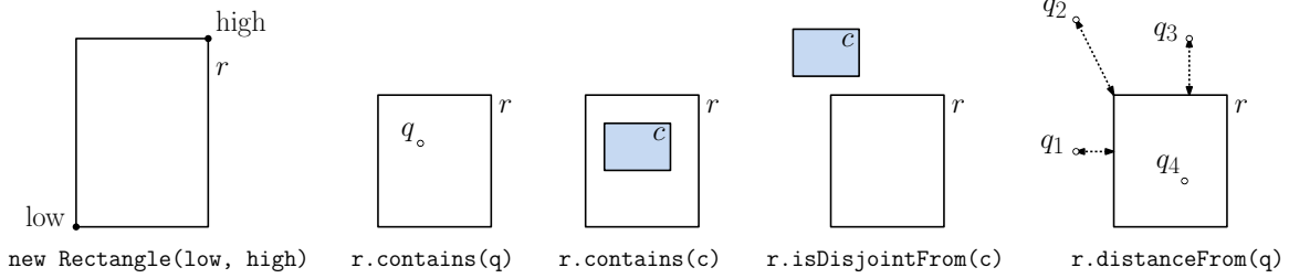
Fig. 79: An axis-parallel rectangle methods.
