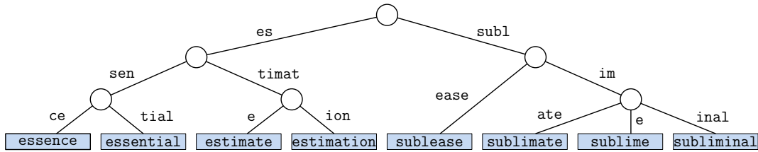
Fig. 114: Alternative (but equivalent) method of drawing the patricia trie of Fig. 113.
