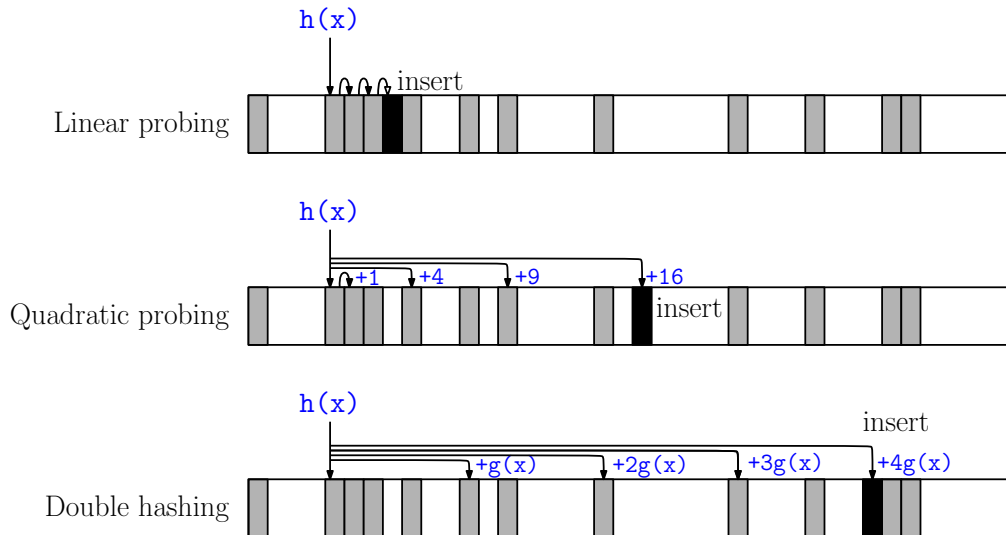
Fig. 97: Various open-addressing systems. (Shaded squares are occupied and the black square indicates where the key is inserted.)
