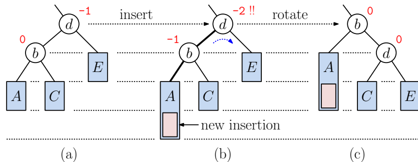
Fig. 36: Restoring balance after insertion through a single rotation.
