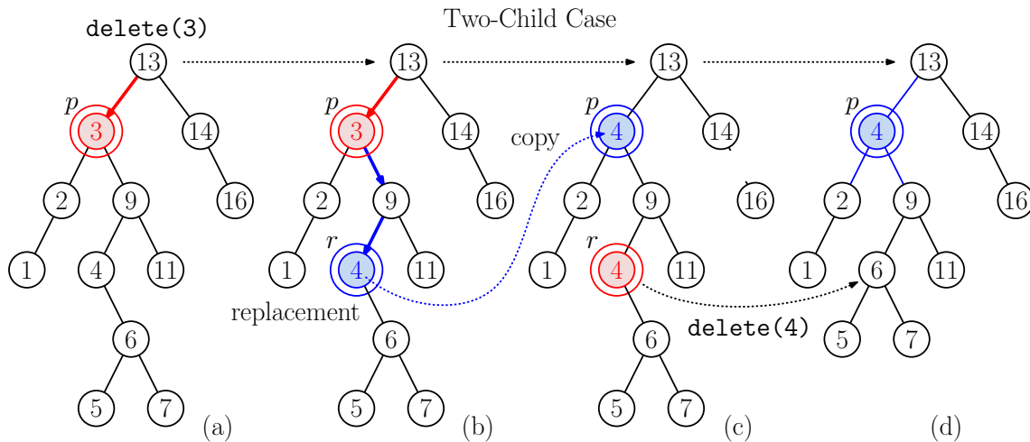
Fig. 30: Deletion: Two-child case.
