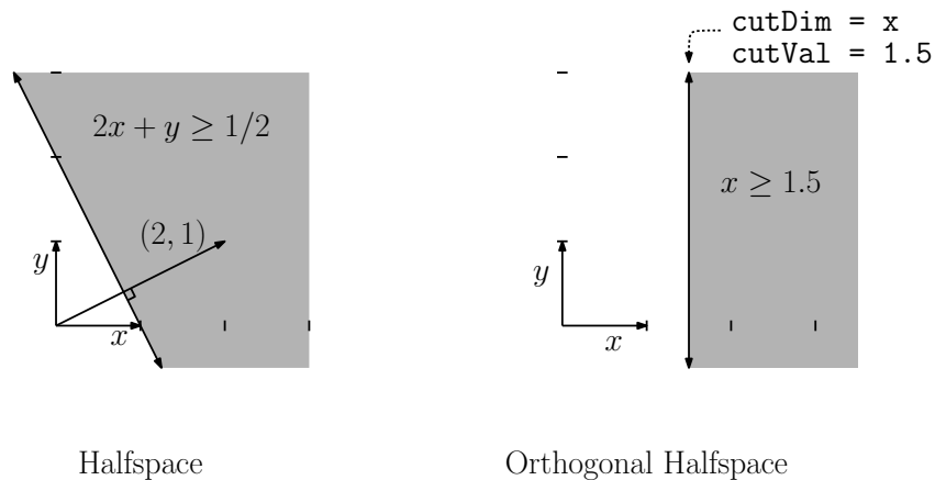
Fig. 133: Planes and Halfspaces.
