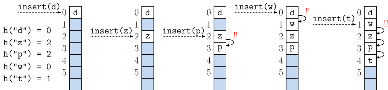
Fig. 96: Linear probing.
