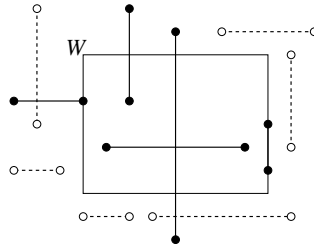
Fig. 139: Window Query.
