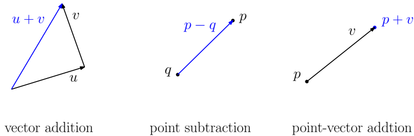
Fig. 136: Point-vector operators.
