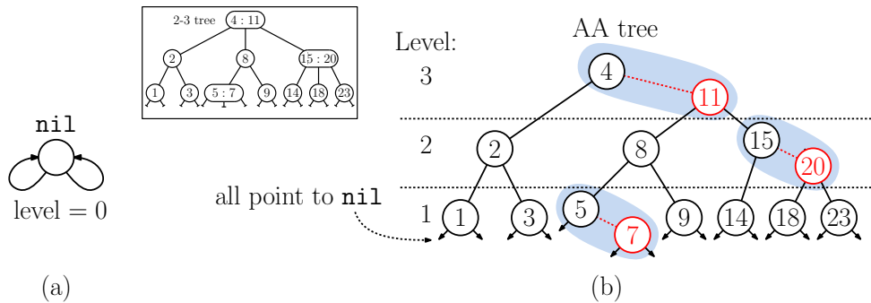
Fig. 48: AA trees: (a) the nil sentinel node, (b) the AA tree for a 2-3 tree.
