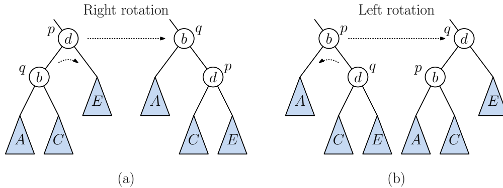
Fig. 34: (Single) Rotations. (Triangles denote subtrees, which may be null.)
