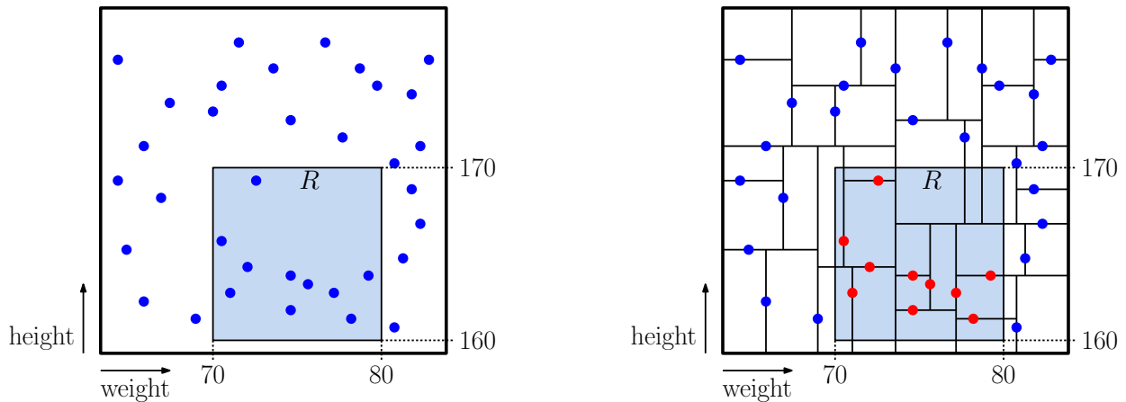
Fig. 78: Orthogonal range query.
