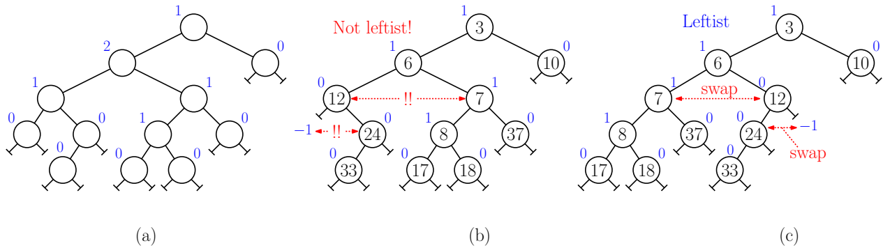
Fig. 23: Null path lengths and the leftist property.
