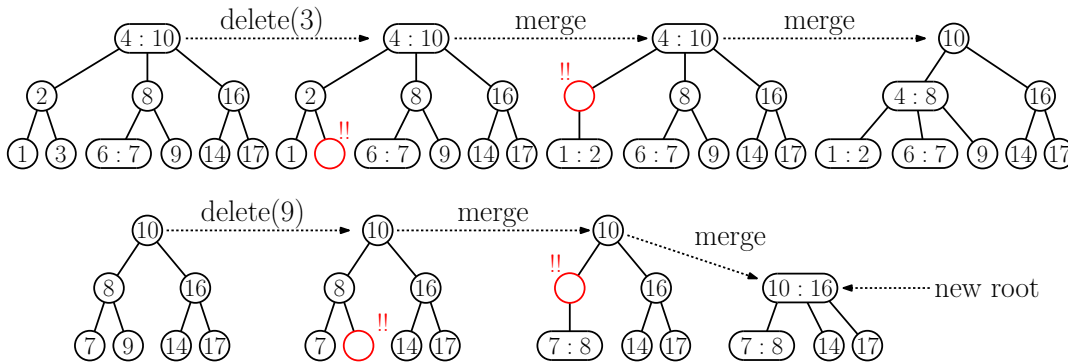
Fig. 45: Two more examples of 2-3 tree deletions.
