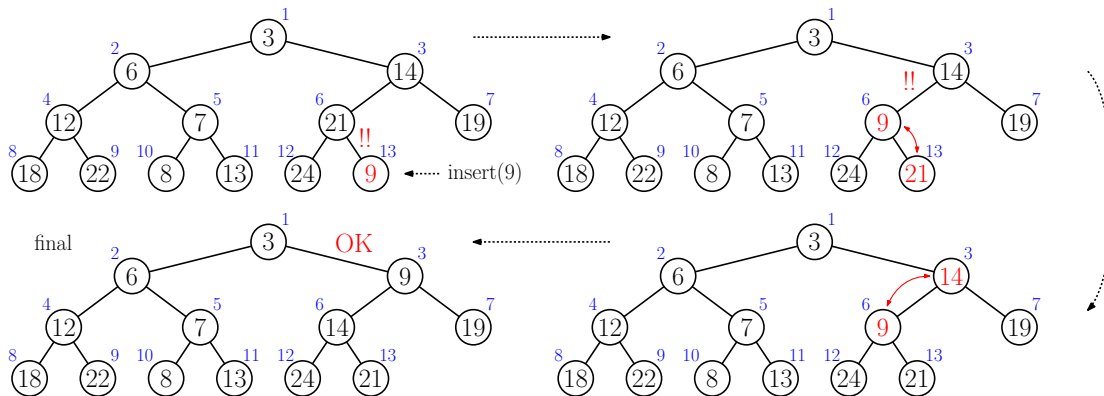
Fig. 21: Example of inserting a new element (9) into a binary heap and sifting up.
