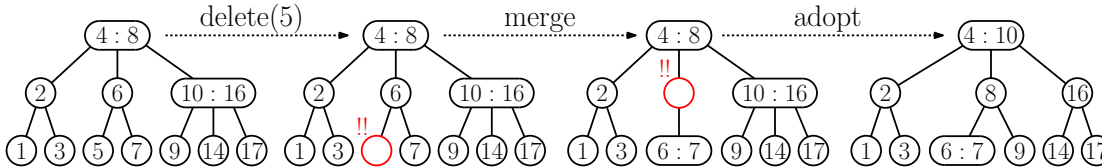
Fig. 44: 2-3 tree deletion involving a merge and an adoption.
