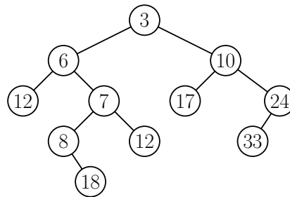
Fig. 19: A (min) heap-ordered binary tree. (Only priorities are shown.)
