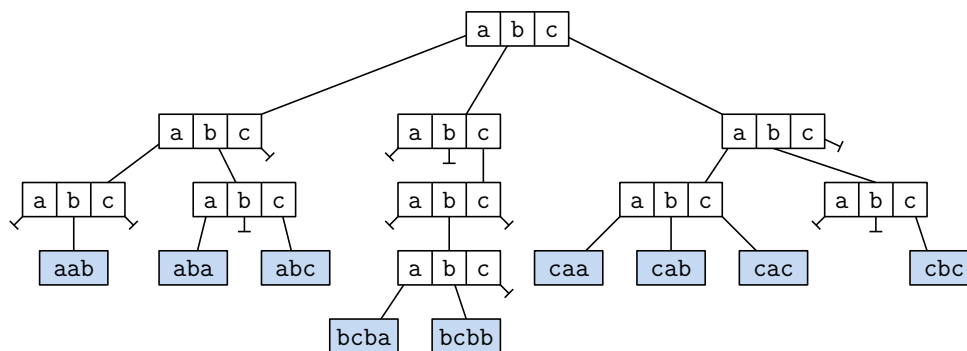
Fig. 109: A trie containing the set \{aab, aba, abc, bcba, bcbb, caa, cab, cac, cbc\} .
