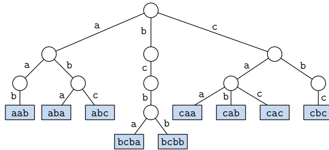
Fig. 110: Alternative (but equivalent) method of drawing the trie of Fig. 109.
