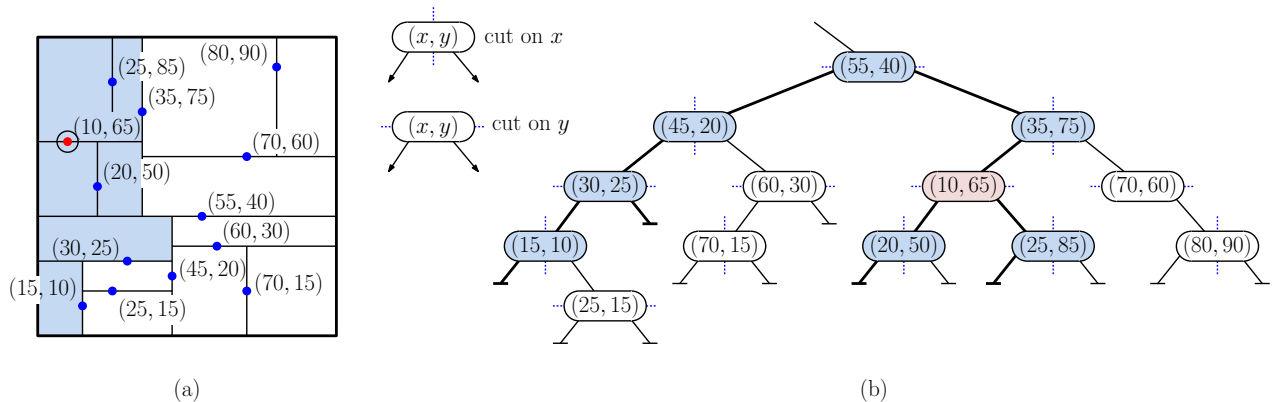
Fig. 76: Example of findMin when i = 0 (the x -coordinate) on the subtree rooted at (55, 40) . The function returns (10, 65) .
