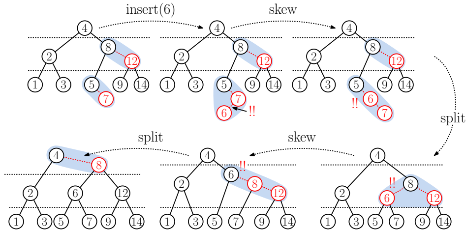
Fig. 51: Example of AA-tree insertion. (Remember, a node is red if it is at the same level as its parent.)
