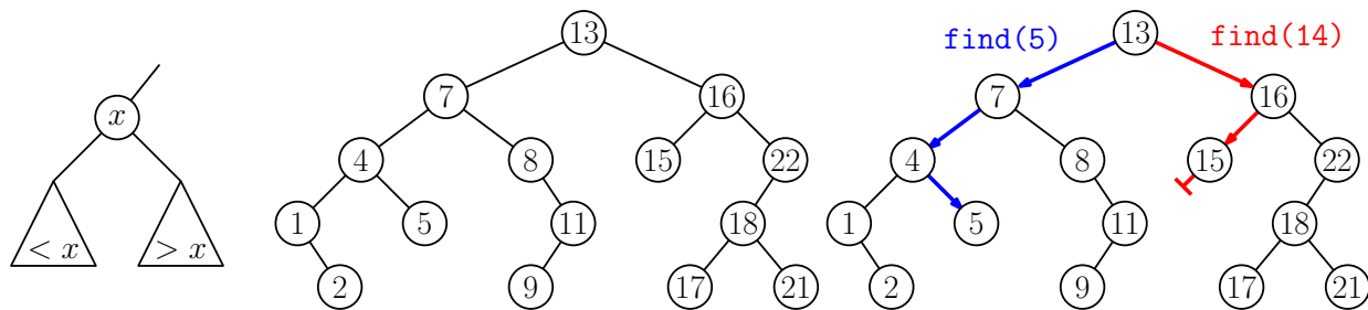
Fig. 26: A possible binary search tree for the key set \{1, 2, 4, 5, 7, 8, 9, 11, 13, 15, 16, 17, 18, 21, 22\} and the search paths for find(5) and find(14) .
