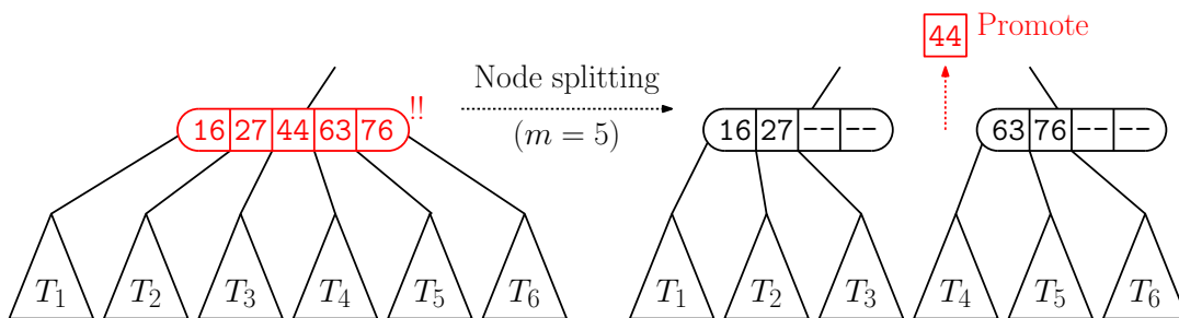
Fig. 103: Node splitting for a B-tree of order m = 5 .
