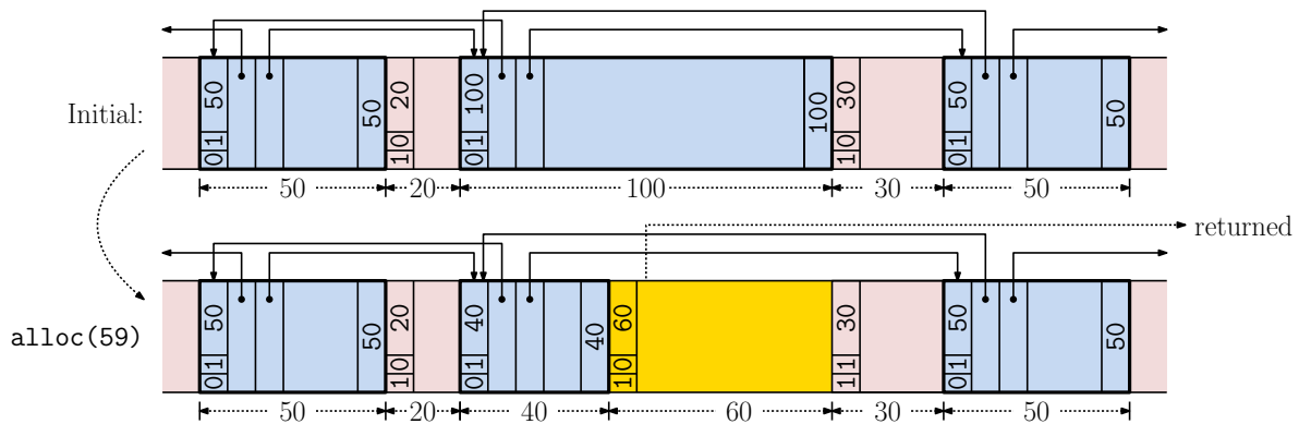
Fig. 119: An example of block allocation.
