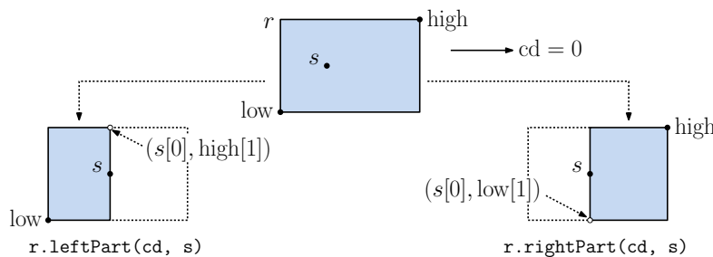
Fig. 80: The functions leftPart and rightPart .
