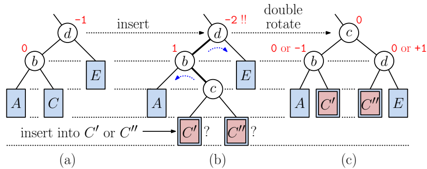
Fig. 37: Restoring balance after insertion through a double rotation.
