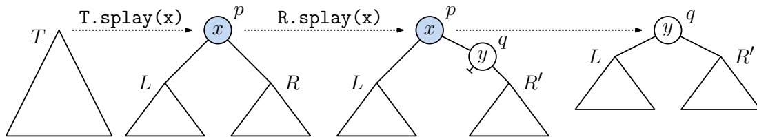
Fig. 69: Splay-tree deletion of x .
