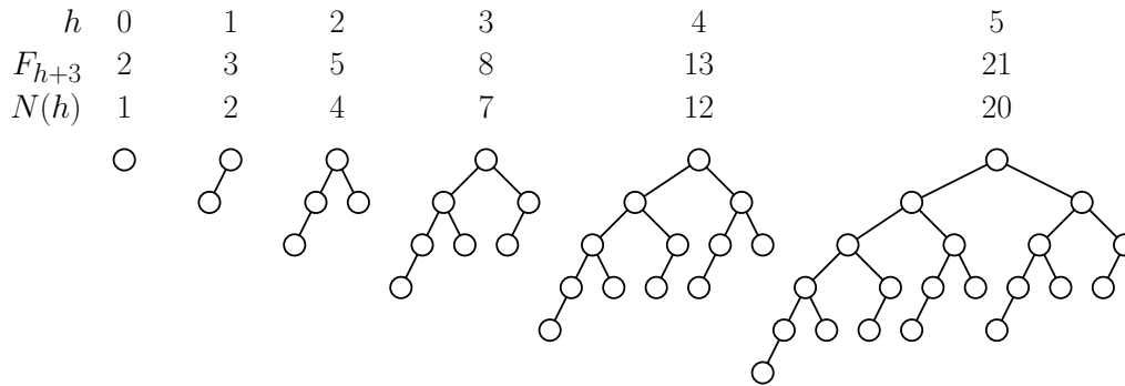
Fig. 33: Minimal AVL trees and Fibonacci numbers.
