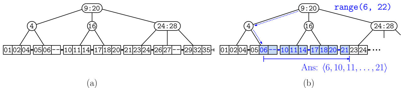
Fig. 108: B+ tree of order m = 3 , where leaves can hold up to 3 keys.
