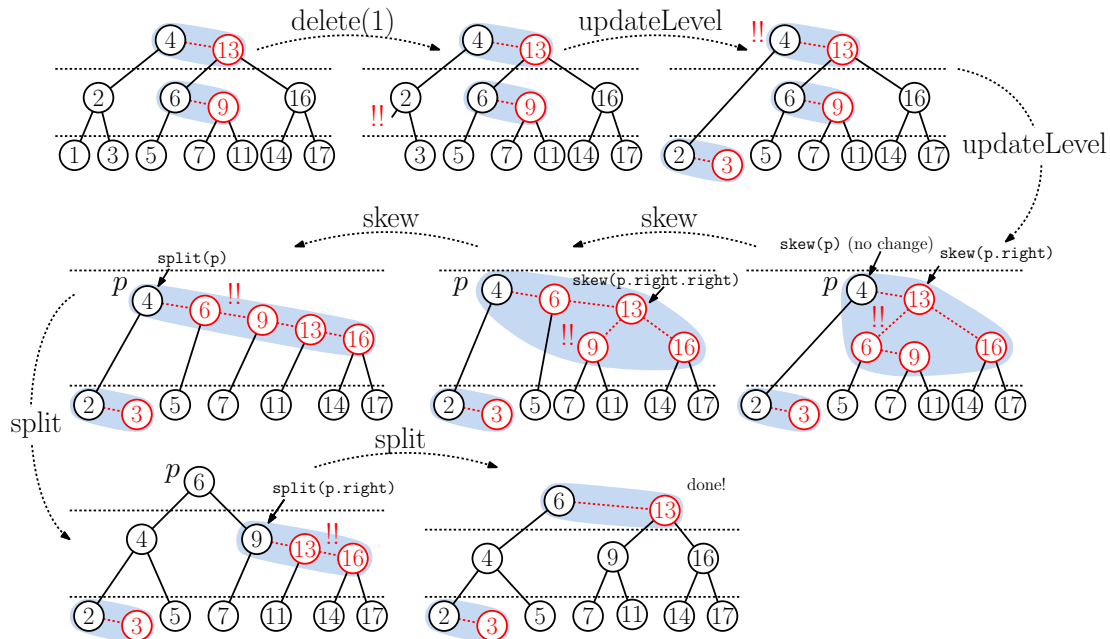
Fig. 52: Example of AA-tree deletion. (Remember, a node is red if it is at the same level as its parent.)
