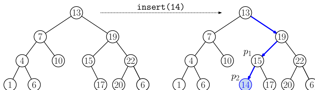
Fig. 28: Binary tree insertion.
