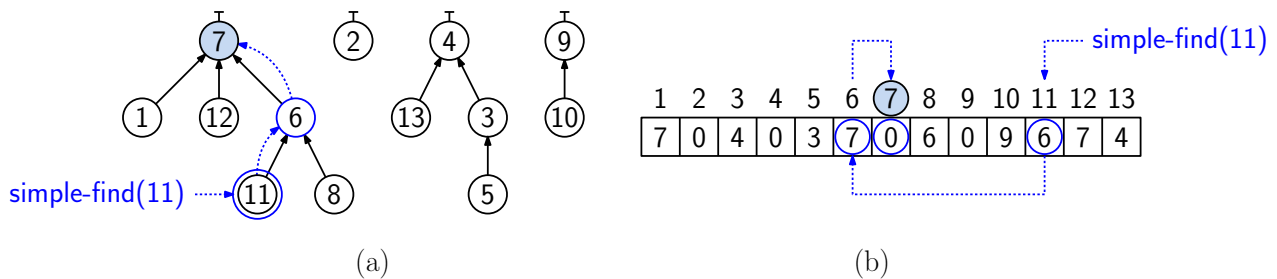
Fig. 15: The operation \text{simple-find}(11) .
