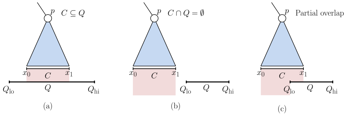
Fig. 92: Range search cases: (a) Q contains p 's cell, (b) Q is disjoint from p 's cell, (c) Q partially overlaps p 's cell.
