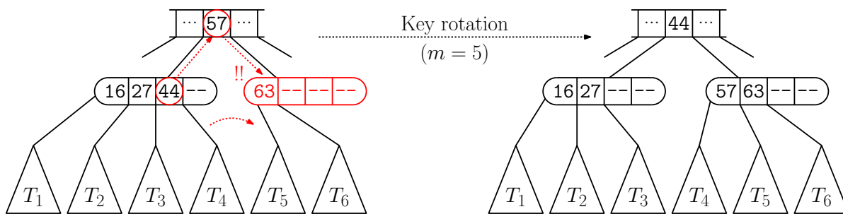
Fig. 102: Key rotation for a B-tree of order m = 5 .
