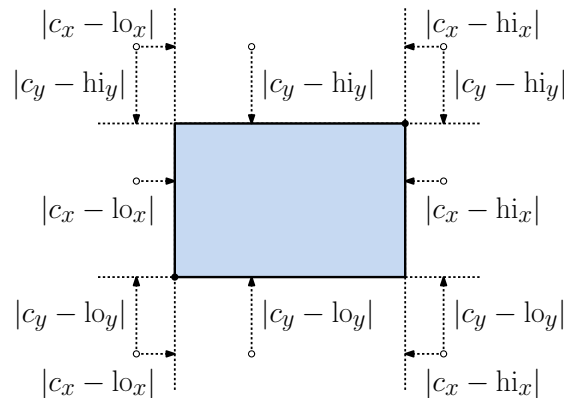
Fig. 138: Distance from a point to a rectangle, and squared distance contributions for each region.
