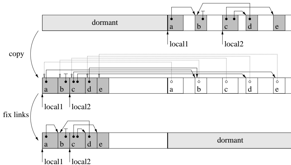
Fig. 145: Stop-and-copy and pointer redirection.
