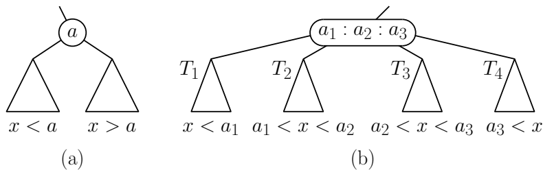
Fig. 100: Binary and 4-ary search tree nodes.
