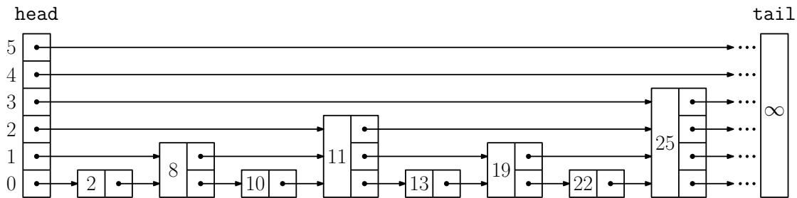
Fig. 57: The “ideal” skip list.
