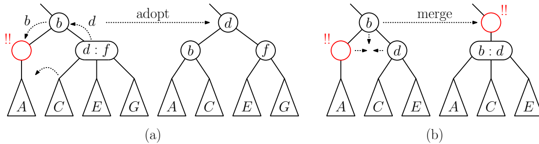
Fig. 43: 2-3 tree deletion: (a) adopting a key/subtree from a sibling and (b) merging two nodes.
