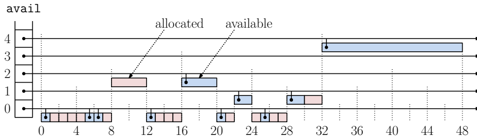
Fig. 122: Buddy system example. Allocated blocks are shaded red and available blocks are shaded blue. Available blocks are linked into the available-block list of the appropriate size.
