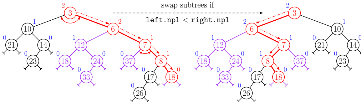
Fig. 25: Merging leftist heaps (Phase-2): Swap left-right to restore leftist property.
