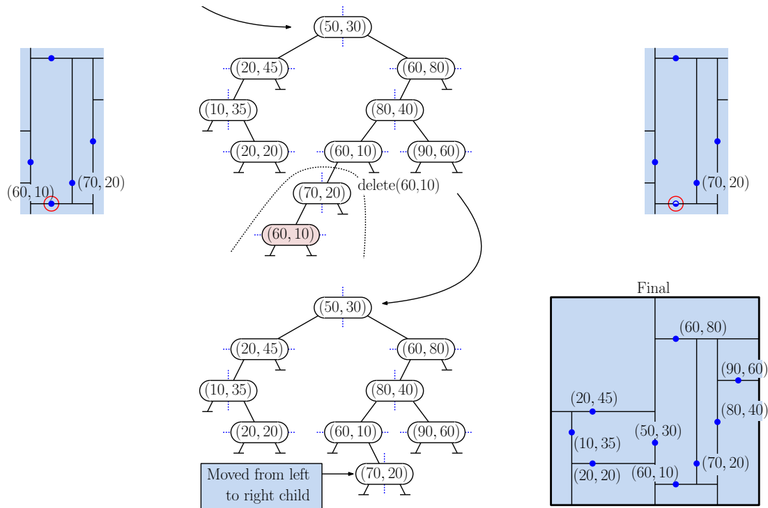
Fig. 77: Deletion from a kd-tree.
