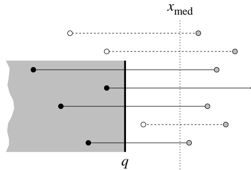
Fig. 142: The segments that stab q lie within the shaded semi-infinite rectangle.
