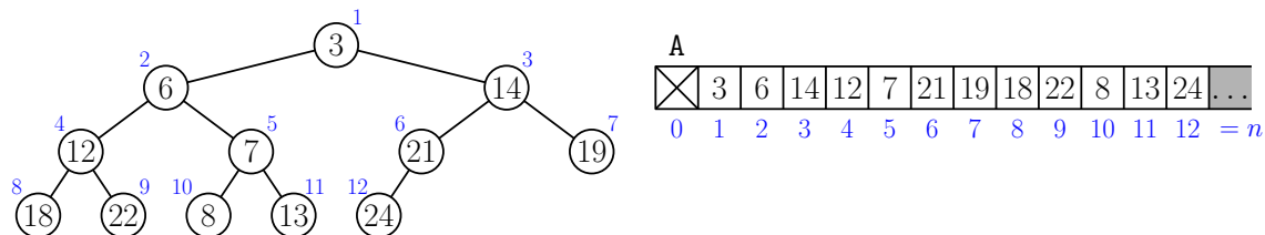
Fig. 20: A heap-ordered complete binary tree and its mapping to an array.
