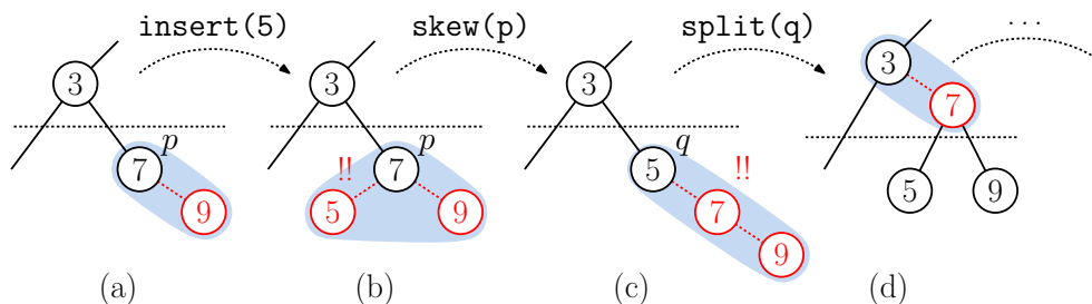
Fig. 50: AA insertion: (a) Initial tree, (b) after insertion, (c) after skewing, (d) after splitting.
