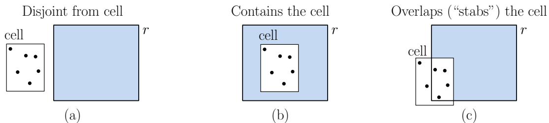
Fig. 81: Cases arising in orthogonal range searching.
