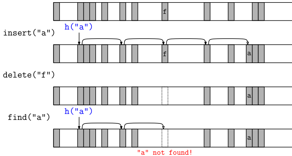
Fig. 98: The problem with deletion in open addressing systems.
