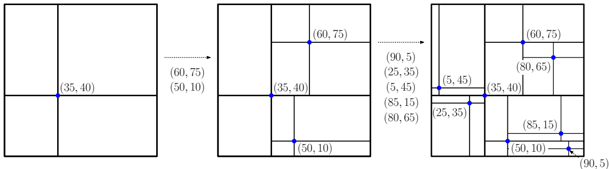
Fig. 71: Point quadtree subdivision.
