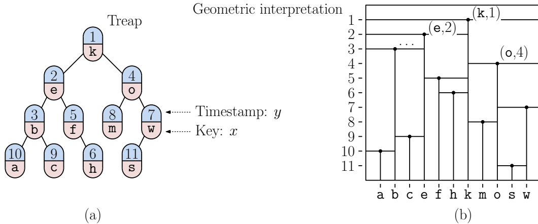
Fig. 54: (a) A treap and (b) geometric interpretation as a (randomized) priority search tree.
