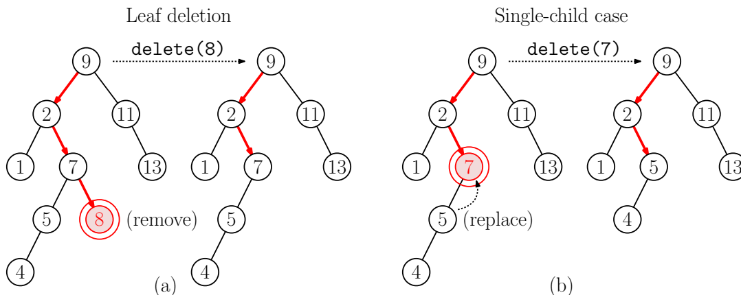
Fig. 29: Deletion: (a) Leaf and (b) single-child case.
