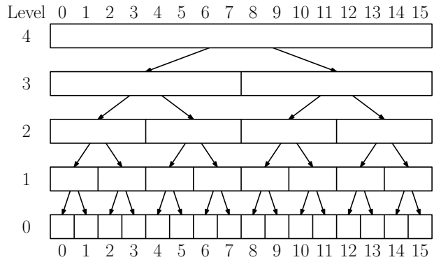
Fig. 121: Buddy system block structure.
