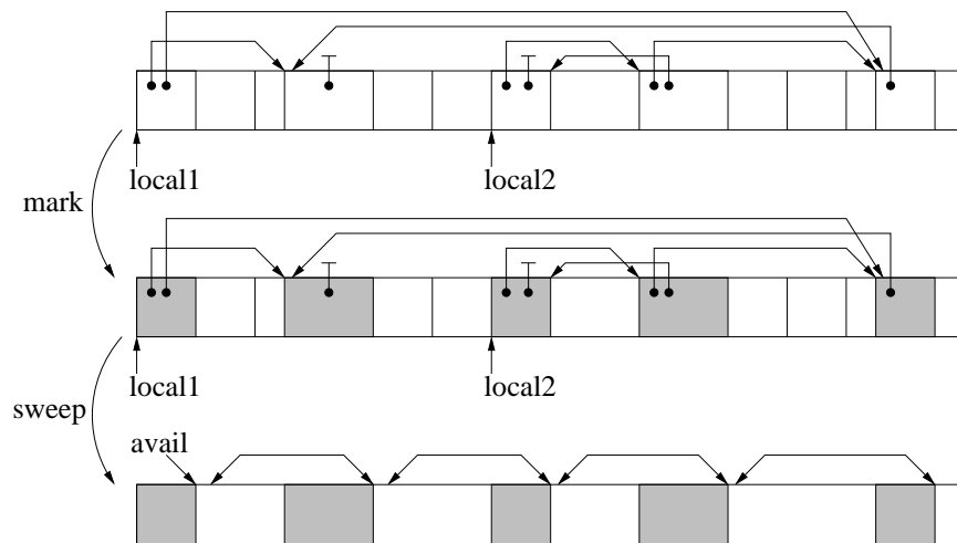
Fig. 143: Mark-and-sweep garbage collection.
