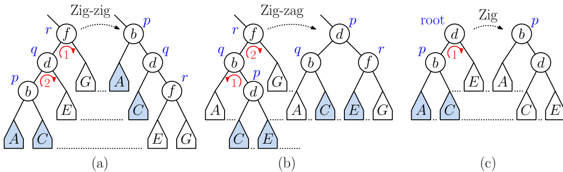
Fig. 66: Splaying cases: (a) Zig-Zig, (b) Zig-Zag and (c) Zig.
