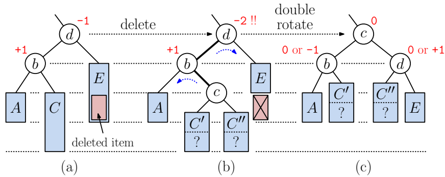
Fig. 39: Restoring balance after deletion with double rotation.
