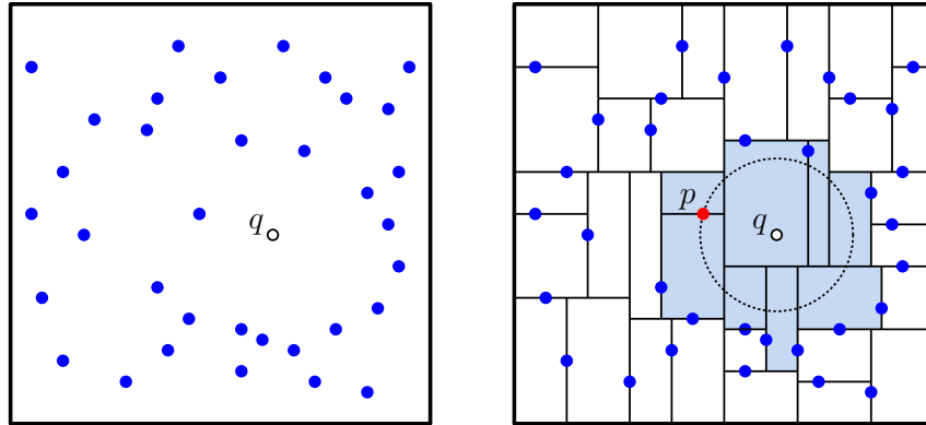
Fig. 84: Nearest-neighbor searching using a kd-tree.
