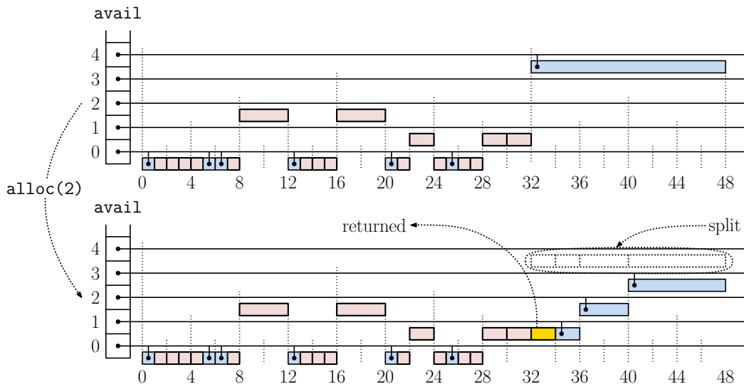
Fig. 123: Example of allocating a block in the buddy system.
