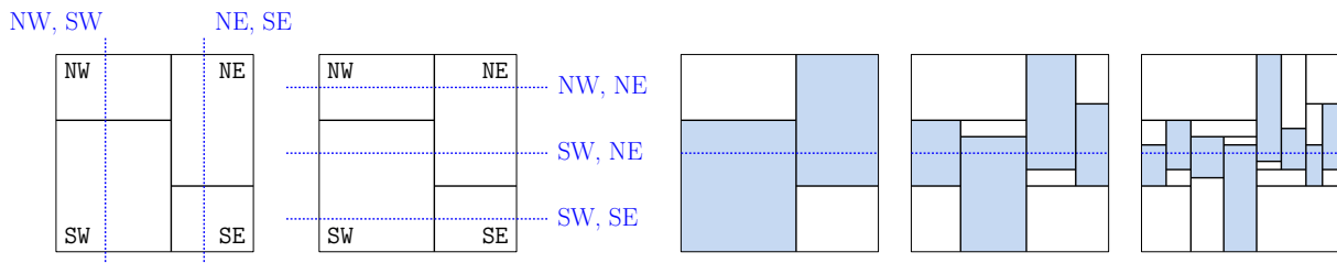
Fig. 83: An axis-parallel line in 2D can stab at most two out of four cells in two levels of the kd-tree decomposition. In general, it stabs 2^i cells at level 2i .
