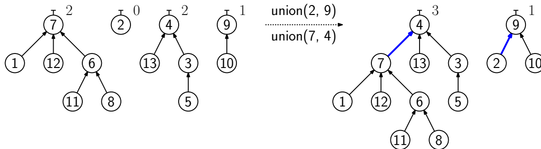
Fig. 16: Union-find with ranks.
