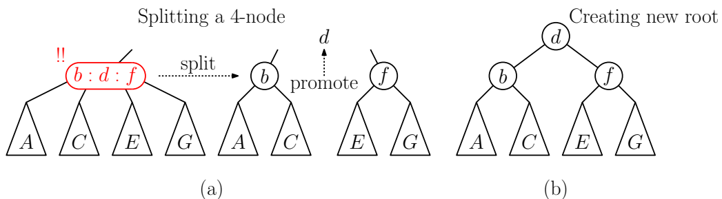
Fig. 41: 2-3 tree insertion: (a) splitting a 4-node into two 2-nodes and (b) creating a new root.
