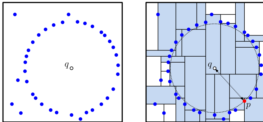
Fig. 85: A (nearly) worst-case scenario for nearest-neighbor searching. Almost all the nodes of the tree need to be visited, since any might be the nearest neighbor.
