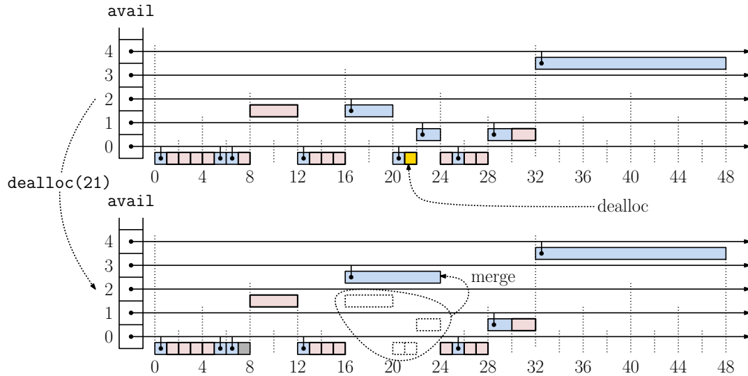
Fig. 124: Example of deallocating a block in the buddy system.
