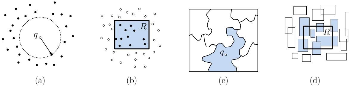
Fig. 70: Common geometric queries: (a) nearest-neighbor searching, (b) range searching, (c) point location, (d) intersection searching.
