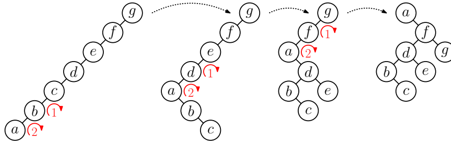
Fig. 65: Two-at-a-time rotations up to the root—the tree height is cut almost in half.
