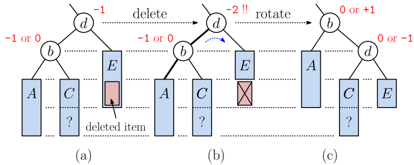
Fig. 38: Restoring balance after deletion with single rotation.
