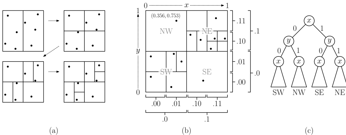
Fig. 116: The PR kd-tree as a digital search tree using bit interleaving.
