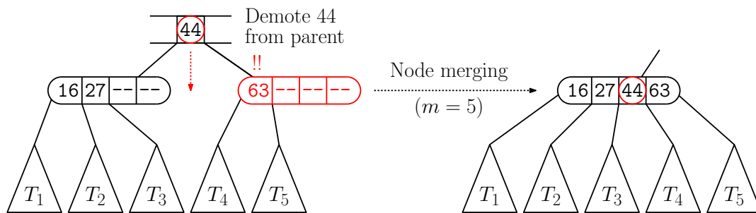
Fig. 104: Node merging for a B-tree of order m = 5 .
