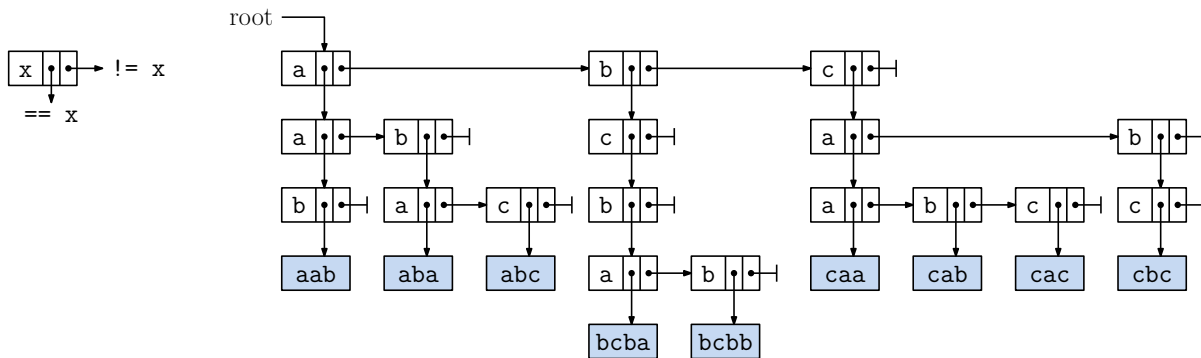
Fig. 111: A de la Briandais tree containing the same strings as in Fig. 109.
