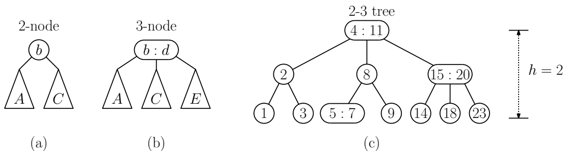
Fig. 40: (a) 2-node, (b) 3-node, and (c) a possible 2-3 tree of height 2.
