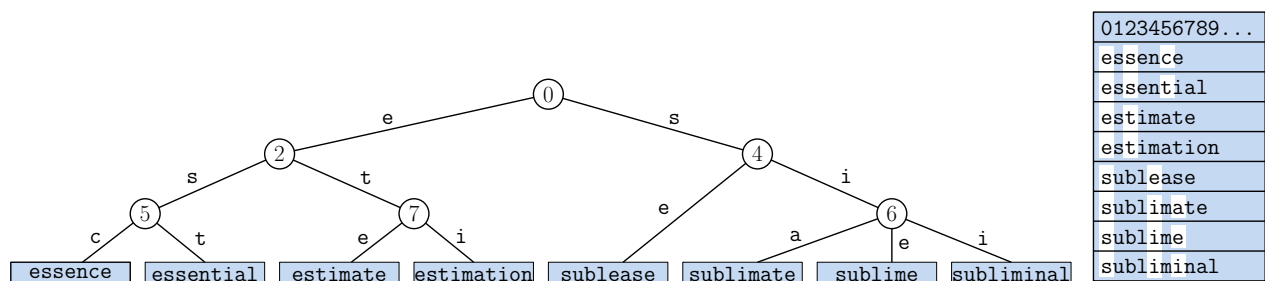
Fig. 113: A patricia trie for a set of strings. Each node is labeled with the index of the character and each edge is labeled with the matching character for this branch.
