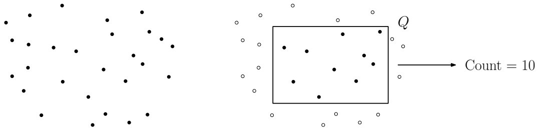
Fig. 88: 2-Dimensional orthogonal range counting query.
