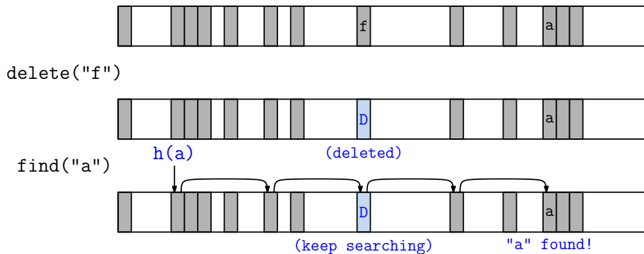
Fig. 99: Deleting in open-addressing by using special empty entry.
