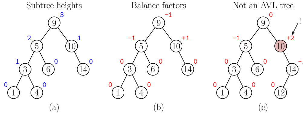
Fig. 32: AVL-tree balance condition.
