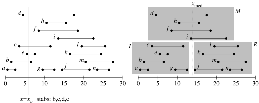
Fig. 140: Line Stabbing Query.
