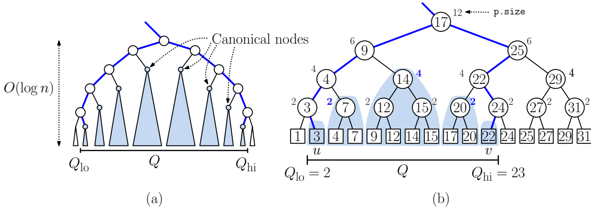
Fig. 91: The canonical subtrees for 1-dimensional range query.
