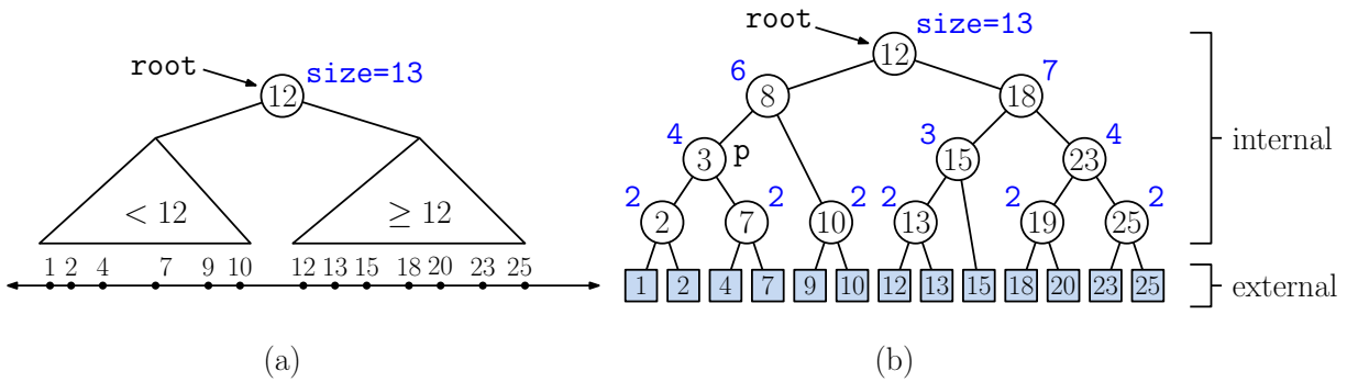
Fig. 89: Extended binary search tree (with sizes).
