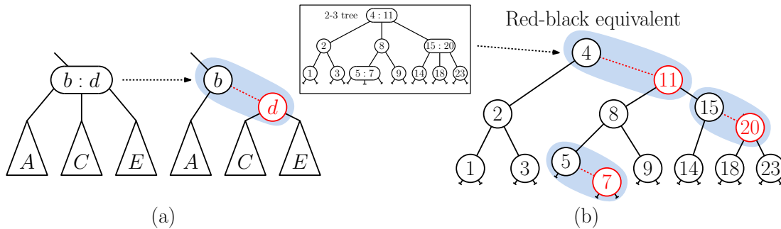
Fig. 46: Encoding a 2-3 tree as an equivalent binary tree.
