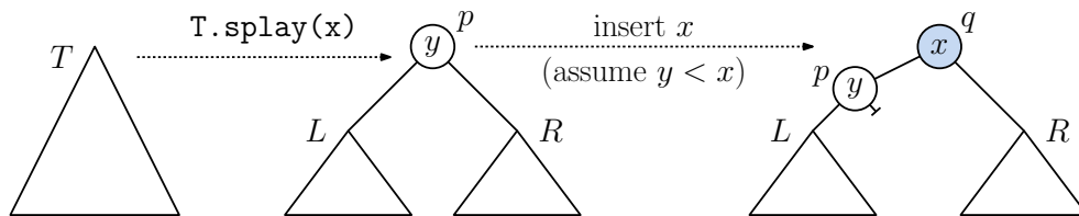
Fig. 68: Splay-tree insertion of x .
