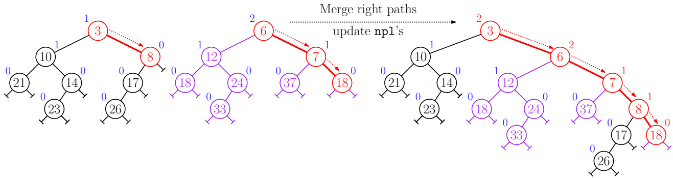
Fig. 24: Merging leftist heaps (Phase-1): Merge rightmost paths by key.
