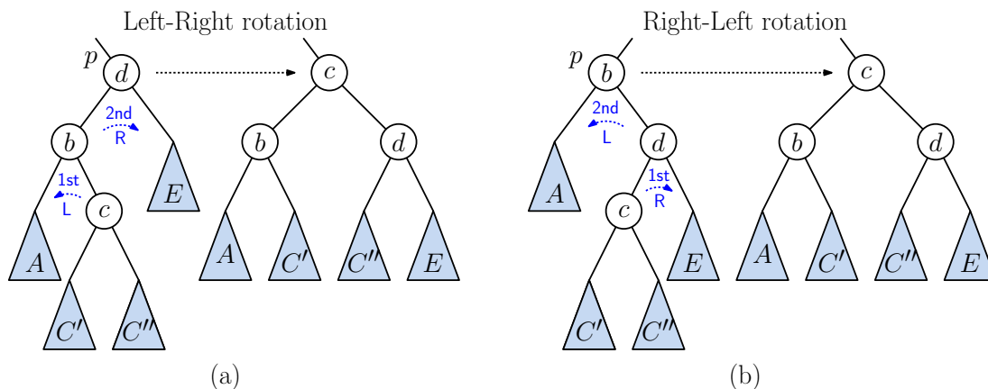
Fig. 35: Double rotations ( rotateLeftRight(p) and rotateRightLeft(p) ).
