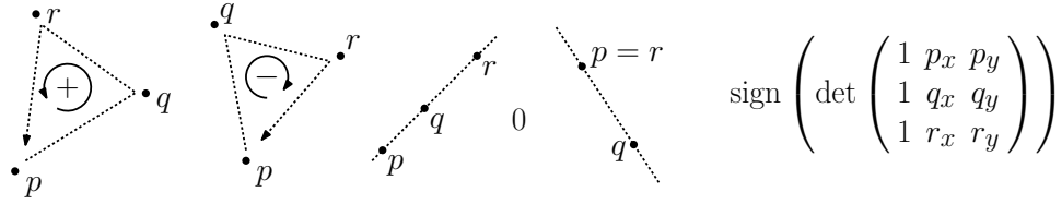
Figure 1: Orientations of the ordered triple (p, q, r) .
