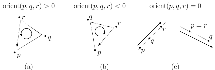
Fig. 6: Orientations of the ordered triple (p, q, r) .
