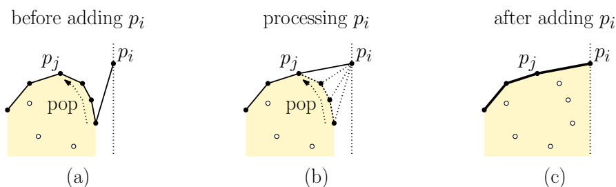
Fig. 7: Graham's scan.
