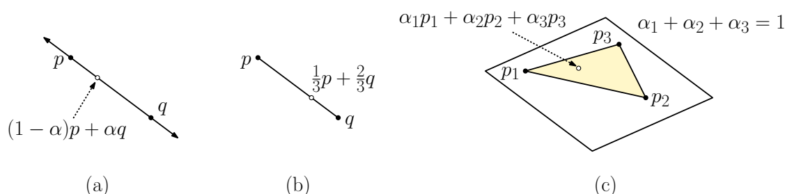
Fig. 2: Affine and convex combinations.
