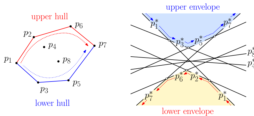
Fig. 6: Equivalence of hulls and envelopes.
