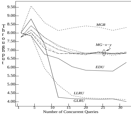
Figure 7: M1, no Data Sharing
