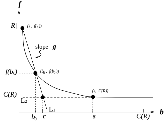
Figure 1: A Typical Faulting Function
