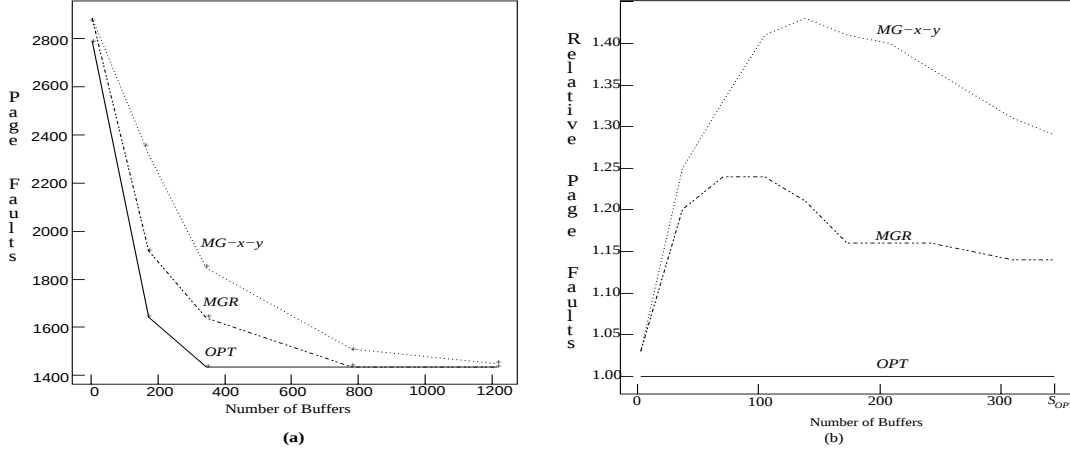
Figure 5: Page Faults Comparison among MGR , MG-x-y and OPT
