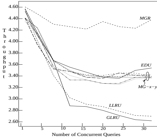
Figure 6: M3, no Data Sharing
