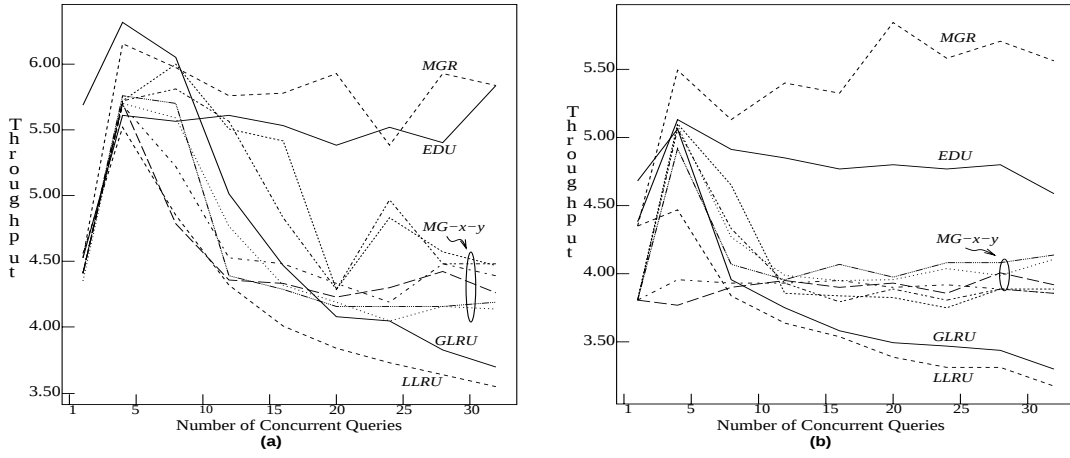
Figure 10: M3, Full Data Sharing, (a) 1000 buffers, (b) 600 buffers
