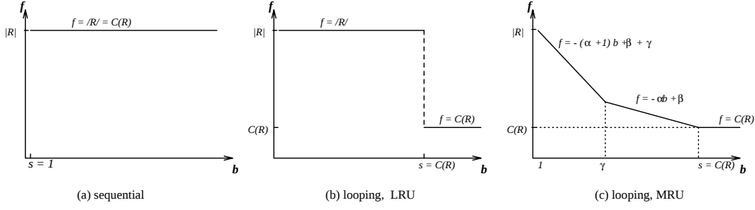
Figure 2: Faulting Functions of Sequential and Looping References
