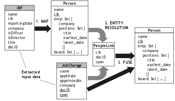
Figure 1: Example Integration Flow
