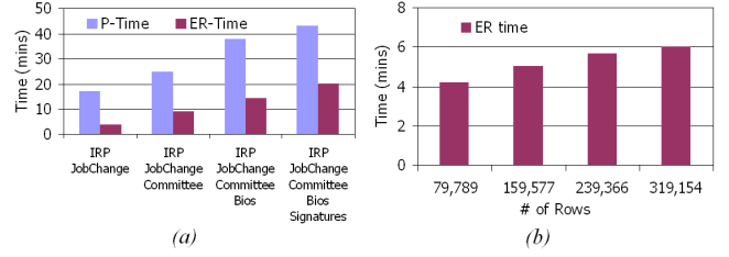
Figure 3: Integration times in the Financial Scenario
