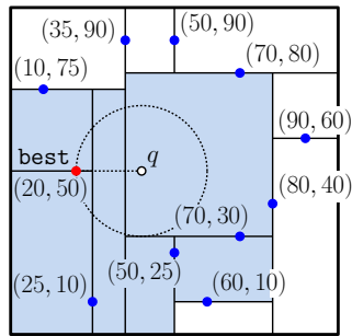
Fig. 86: Nearest-neighbor search.
