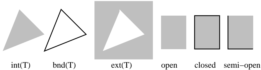
Fig. 128: Topological notation.
