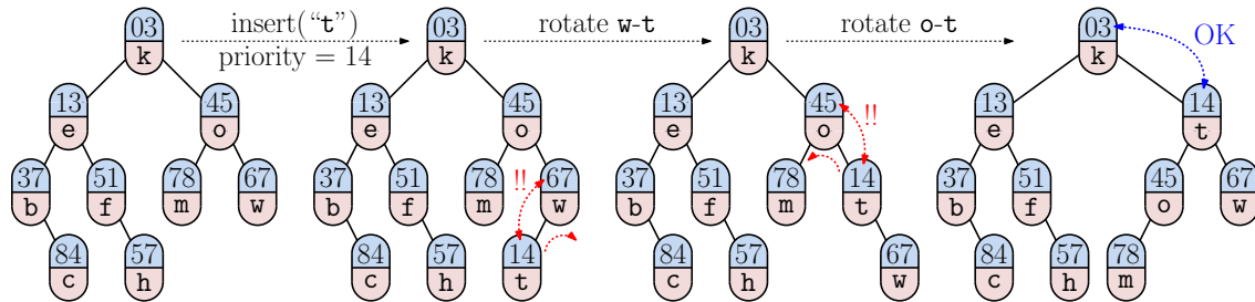
Fig. 43: Treap insertion.
