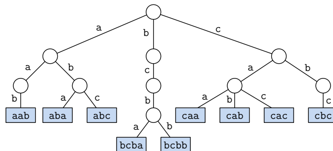
Fig. 100: Alternative (but equivalent) method of drawing the trie of Fig. 99.
