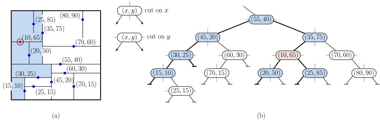
Fig. 75: Example of findMin when i = 0 (the x -coordinate) on the subtree rooted at (55, 40) . The function returns (10, 65) .
