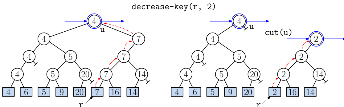
Fig. 122: The operation decrease-key(r, 2) , which decreases key 7 to 2.
