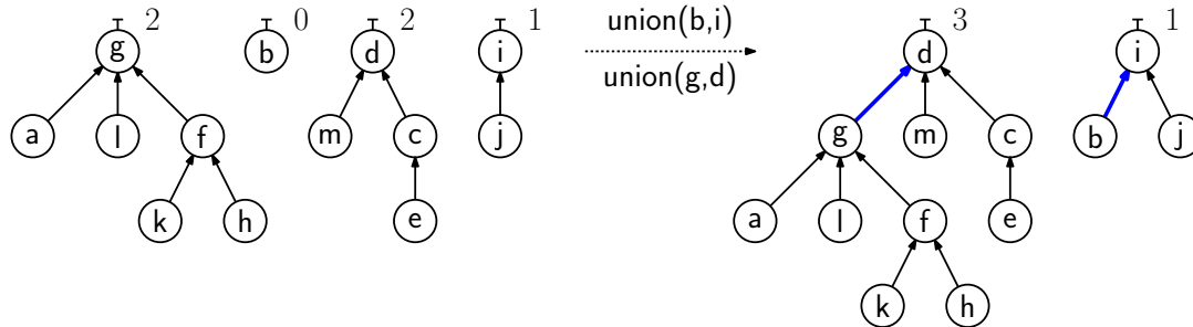
Fig. 116: Union-find with ranks.
