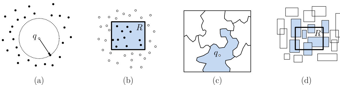
Fig. 69: Common geometric queries: (a) nearest-neighbor searching, (b) range searching, (c) point location, (d) intersection searching.
