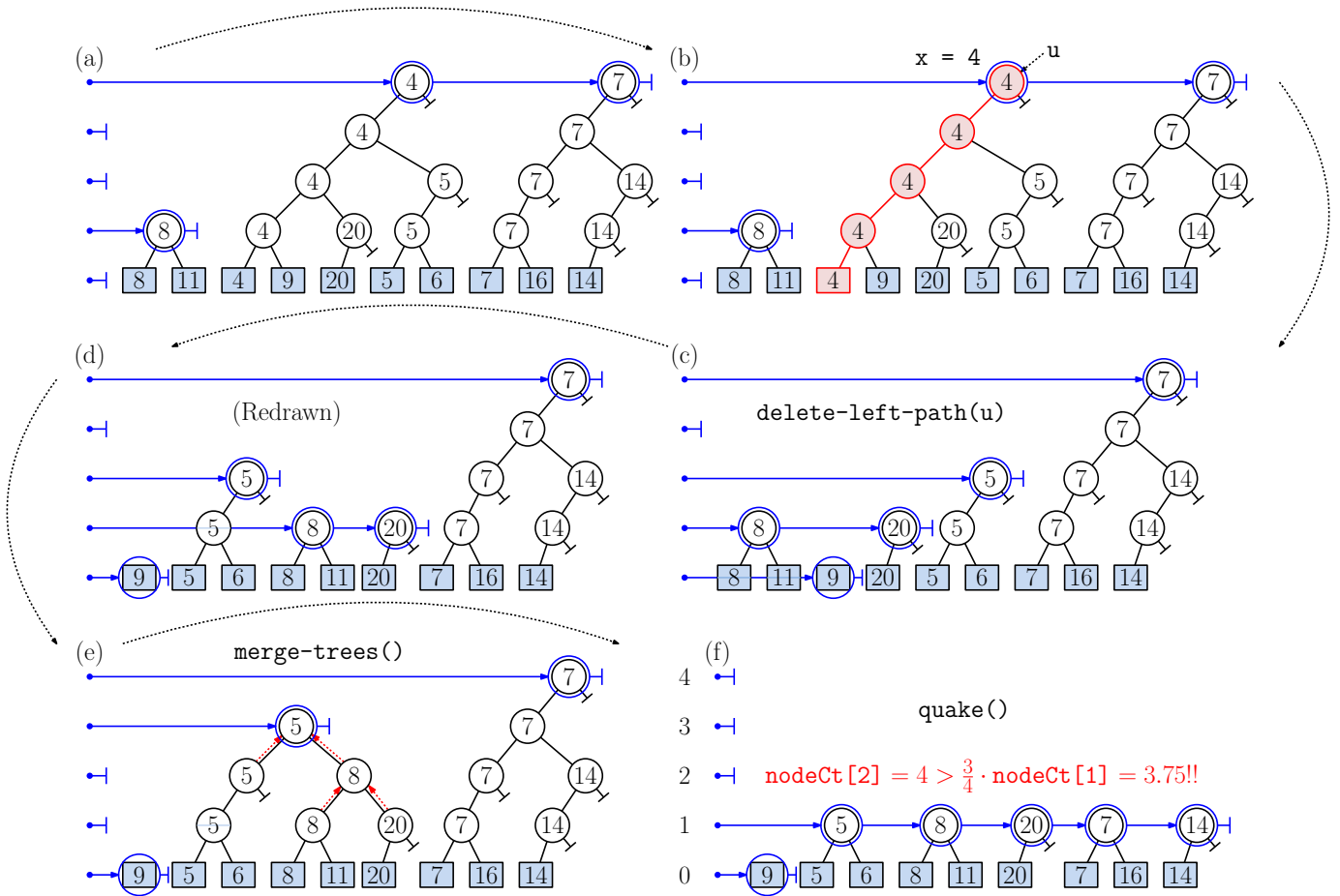
Fig. 123: The operation extract-min() .
