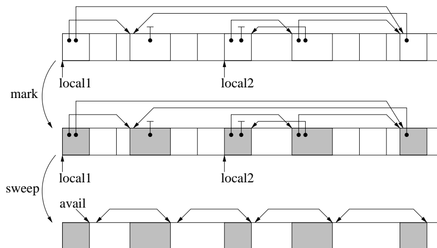
Fig. 136: Mark-and-sweep garbage collection.
