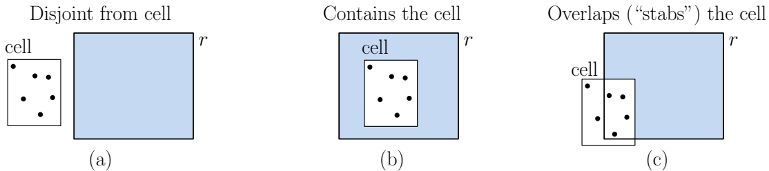
Fig. 80: Cases arising in orthogonal range searching.
