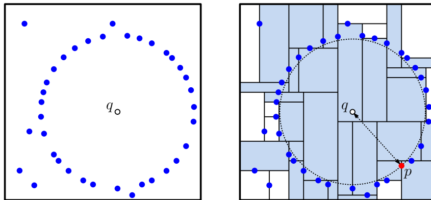
Fig. 84: A (nearly) worst-case scenario for nearest-neighbor searching. Almost all the nodes of the tree need to be visited, since any might be the nearest neighbor.
