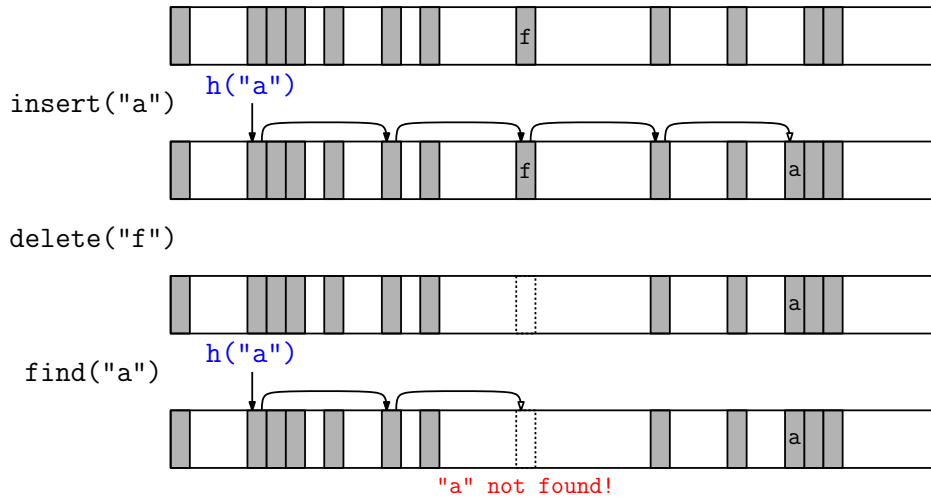
Fig. 91: The problem with deletion in open addressing systems.
