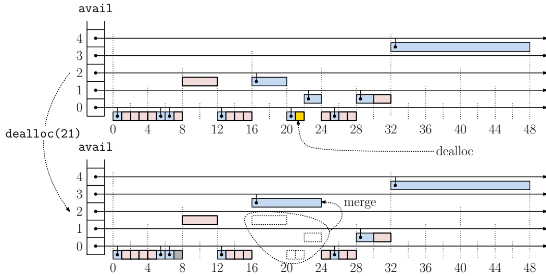
Fig. 114: Example of deallocating a block in the buddy system.
