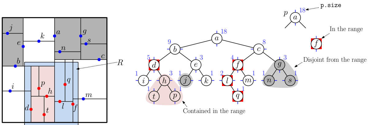
Fig. 81: Range search in kd-trees. The subtree rooted at h is counted entirely. The subtrees rooted at j and g are excluded entirely. The other points are checked individually.
