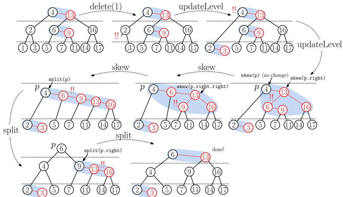
Fig. 40: Example of AA-tree deletion. (Remember, a node is red if it is at the same level as its parent.)
