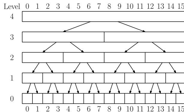
Fig. 111: Buddy system block structure.
