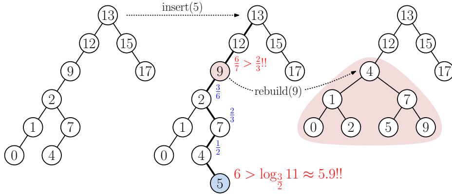
Fig. 68: Inserting a key into a scapegoat tree, which triggers a rebuilding event. The node containing 9 is the first scapegoat candidate encountered while backtracking up the search path and is rebuilt.
