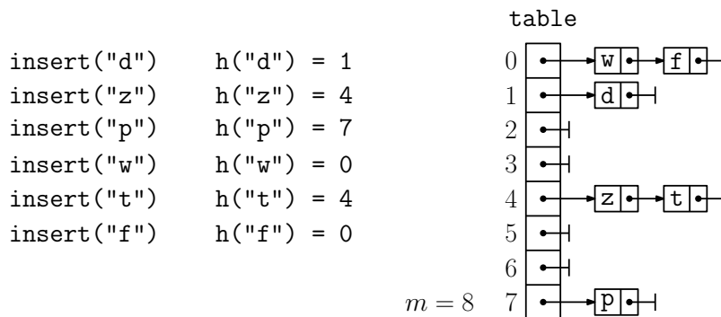
Fig. 87: Collision resolution by separate chaining.
