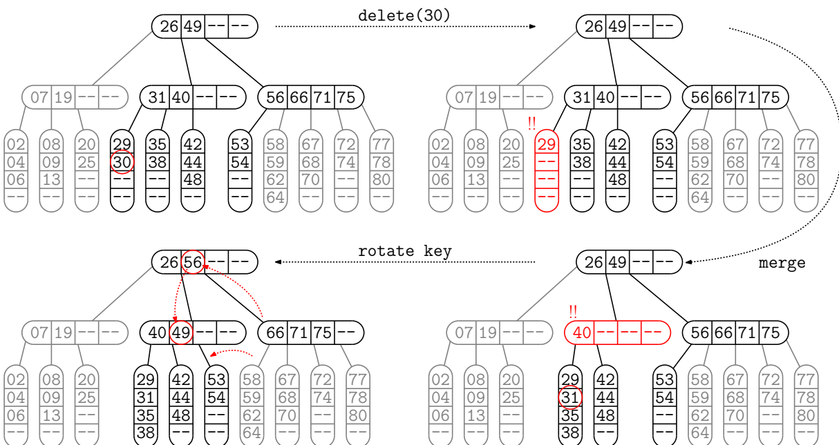
Fig. 65: Deletion of key 30 (order m = 5 ). Its leaf is underfull, but its sibling cannot give up a key, so we merge with (35, 38), demoting the middle key 31 from the parent. Now the parent 40 is underfull, but its right sibling can spare a key, so 56 is rotated to the parent and 49 is rotated down.
