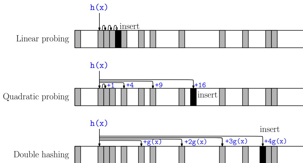
Fig. 90: Various open-addressing systems. (Shaded squares are occupied and the black square indicates where the key is inserted.)
