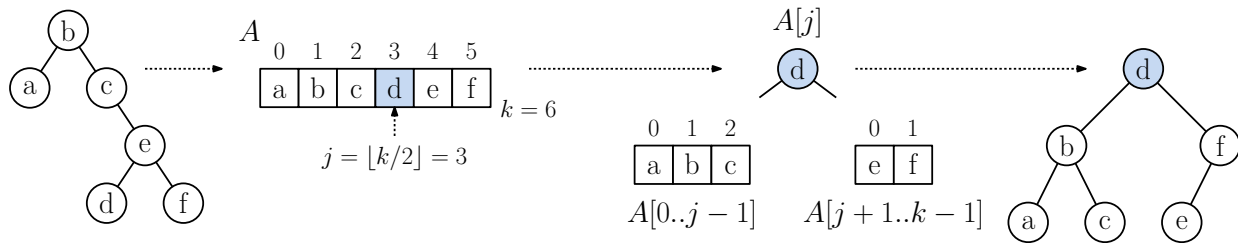
Fig. 67: Recursively building a balanced tree from a sorted array of keys.
