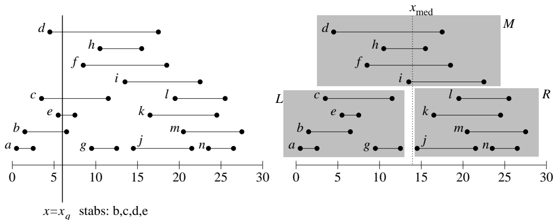
Fig. 133: Line Stabbing Query.
