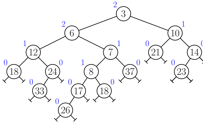
Fig. 118: Leftist heap structure (with npl values shown).
