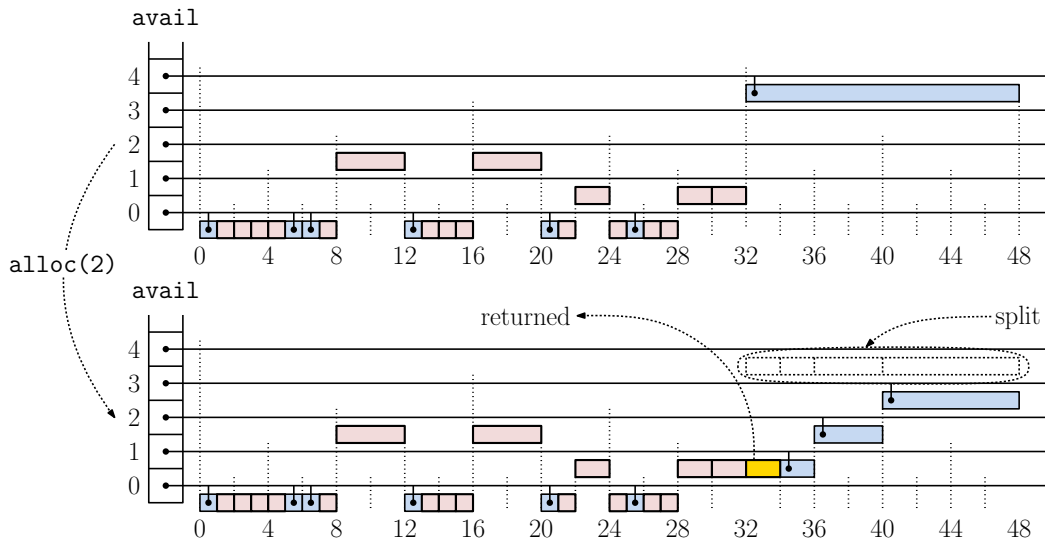
Fig. 113: Example of allocating a block in the buddy system.
