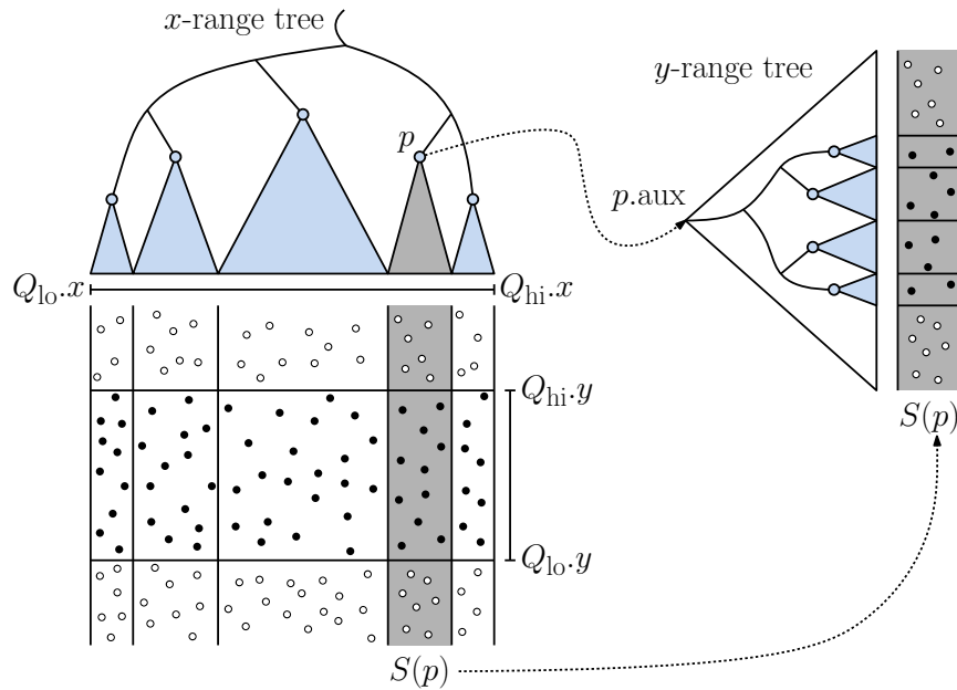
Fig. 98: 2-Dimensional Range tree.
