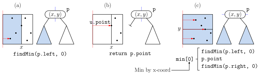
Fig. 74: Cases in findMin .
