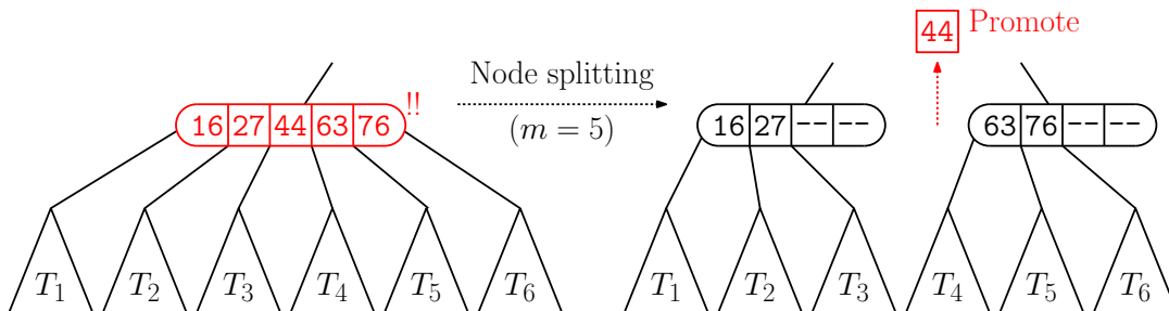
Fig. 61: Node splitting for a B-tree of order m = 5 .
