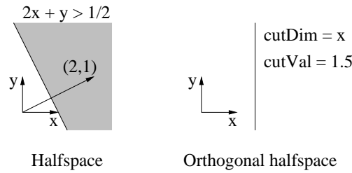
Fig. 126: Planes and Halfspaces.
