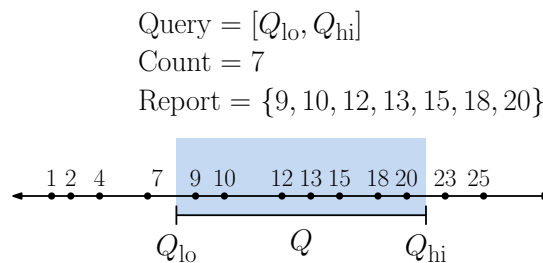
Fig. 95: 1-dimensional range query.
