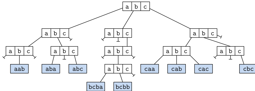
Fig. 99: A trie containing the set \{aab, aba, abc, bcba, bcbb, caa, cab, cac, cbc\} .
