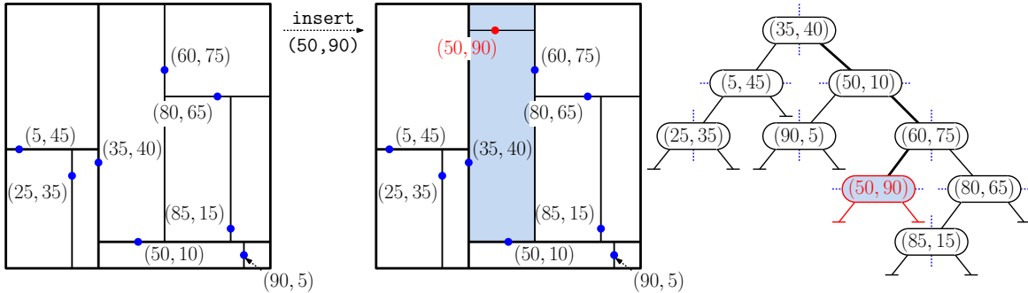
Fig. 73: Inserting (50, 90) into the point kd-tree of Fig. 72.
