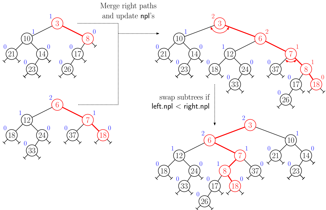
Fig. 119: Example of merging two leftist heaps (2-step interpretation).
