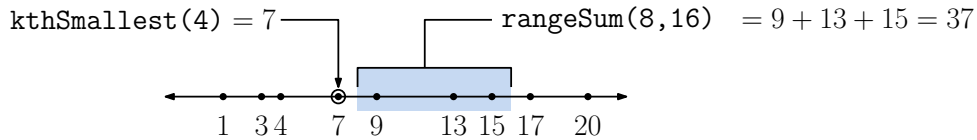
Fig. 50: Order-statistic and range queries.
