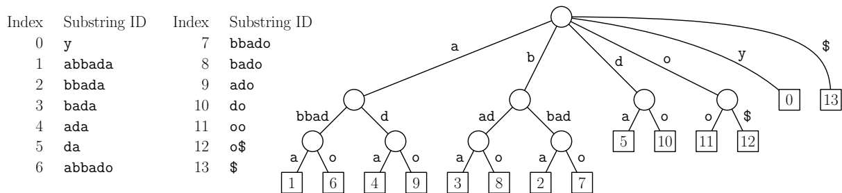
Fig. 105: A suffix tree for the string “ yabbadabbadoo$ ”. (Labels are placed on the edges, but this can be implemented using a standard trie or patricia trie.)
