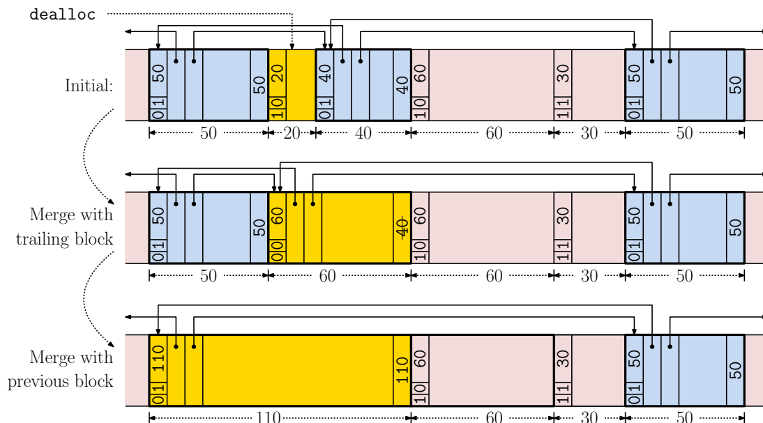
Fig. 110: An example of block deallocation and merging.
