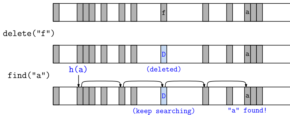
Fig. 92: Deleting in open-addressing by using special empty entry.
