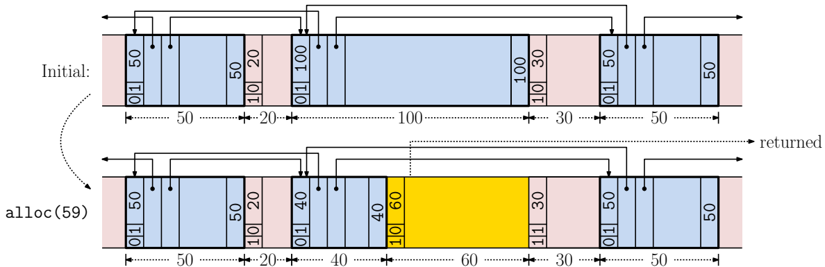
Fig. 109: An example of block allocation.
