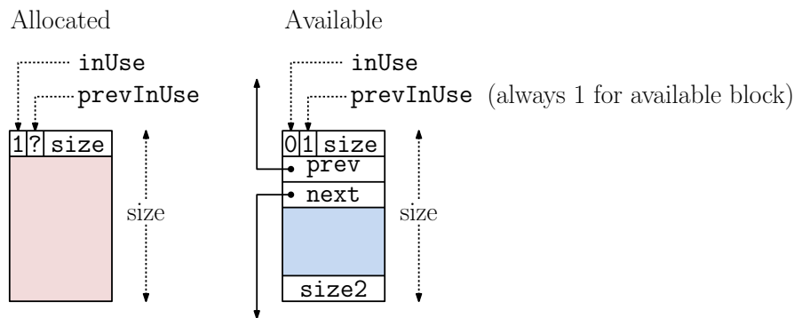
Fig. 108: Block structure for dynamic storage allocation.
