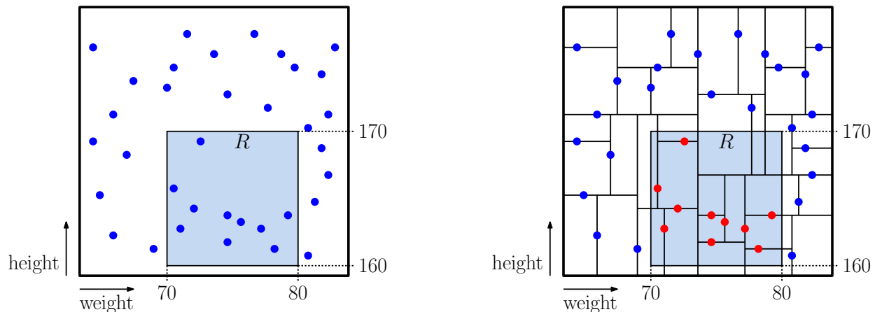
Fig. 77: Orthogonal range query.
