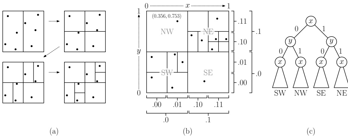
Fig. 106: The PR kd-tree as a digital search tree using bit interleaving.
