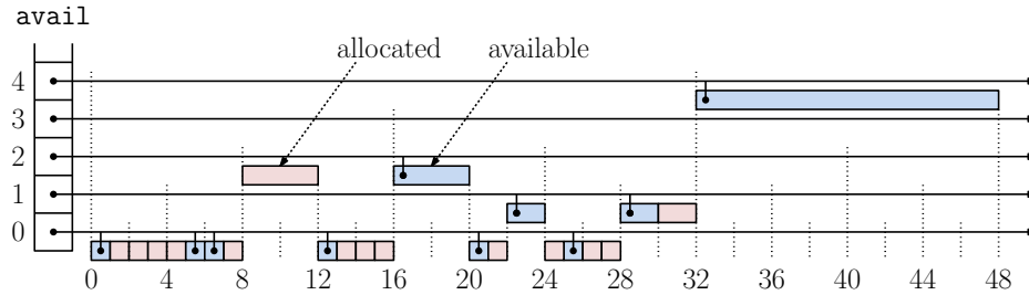
Fig. 112: Buddy system example. Allocated blocks are shaded red and available blocks are shaded blue. Available blocks are linked into the available-block list of the appropriate size.
