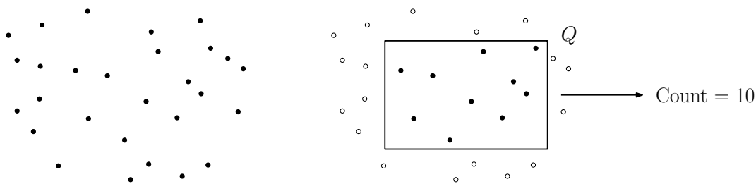
Fig. 93: 2-Dimensional orthogonal range counting query.
