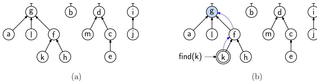
Fig. 115: Union through height-based merging.
