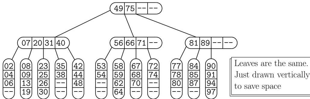
Fig. 59: B-tree of order 5. (Each node, except possibly the root has 3–5 children.)
