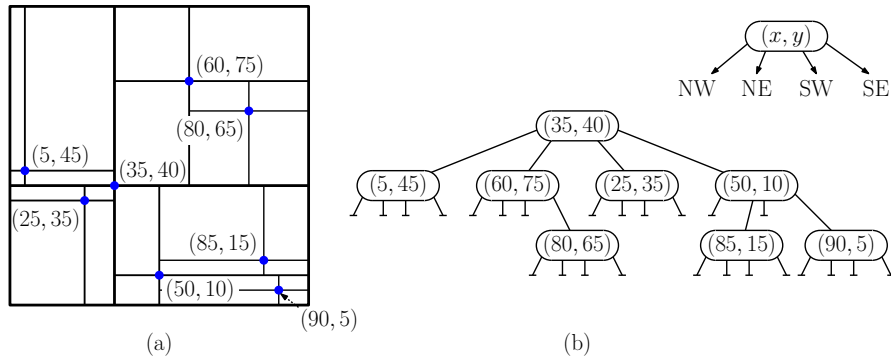
Fig. 71: Point quadtree.
