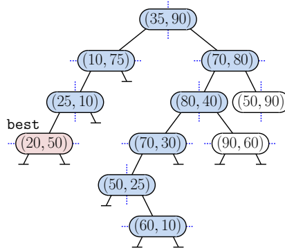
Fig. 86: Nearest-neighbor search.
