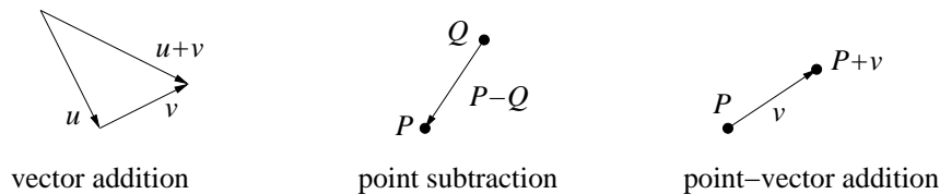
Fig. 129: Point-vector operators.
