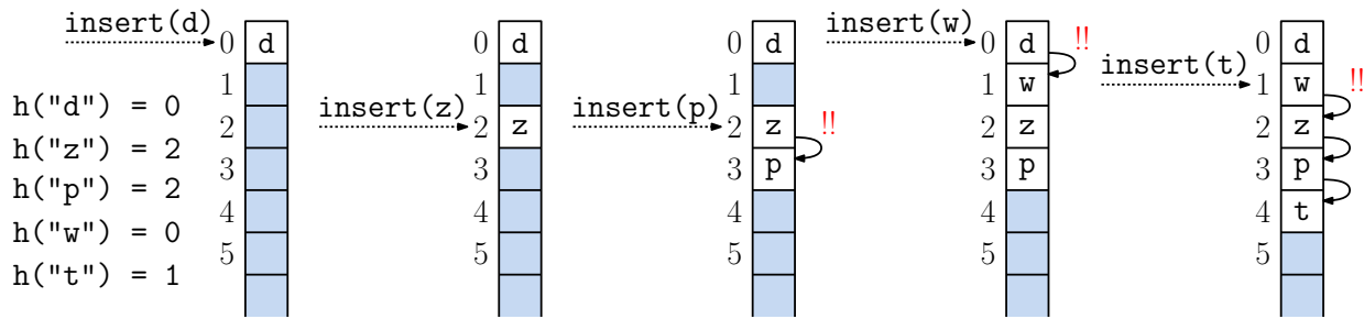
Fig. 89: Linear probing.
