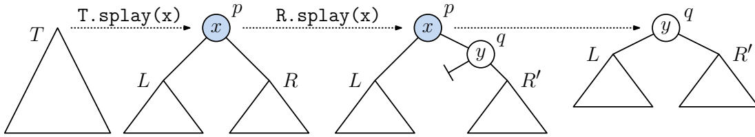
Fig. 57: Splay-tree deletion of x .
