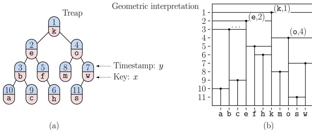
Fig. 42: (a) A treap and (b) geometric interpretation as a (randomized) priority search tree.
