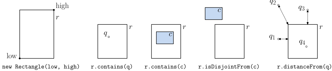
Fig. 78: An axis-parallel rectangle methods.
