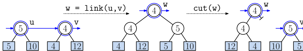
Fig. 121: The operations (a) link and (b) cut.
