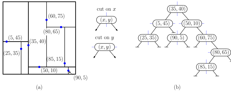
Fig. 72: Point kd-tree decomposition.
