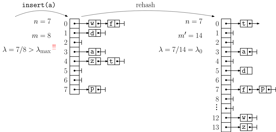
Fig. 88: Controlling the load factor by rehashing, where \lambda_{\min} = 0.25 , \lambda_{\max} = 0.75 , and \lambda_0 = 0.5 . When the table size changes, we create an entirely different hash function.
