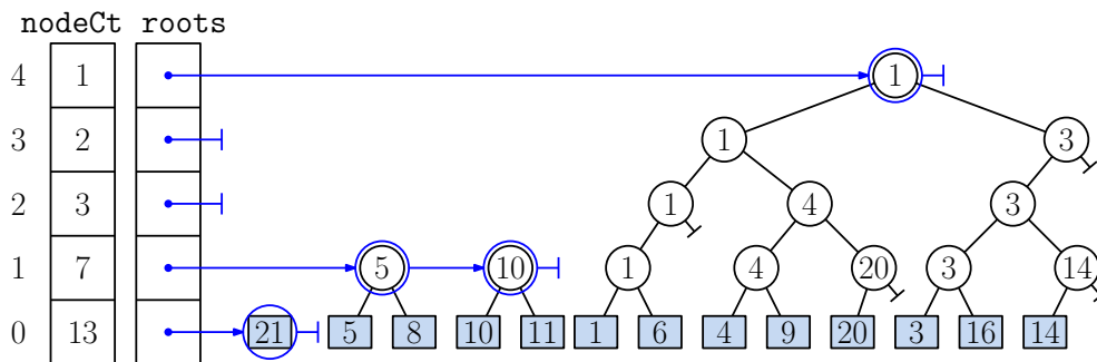
Fig. 120: An example of a quake heap consisting of four trees, storing a total of 13 keys. (As usual, values are omitted.) On the left we show arrays of node counts and roots lists.
