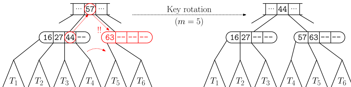
Fig. 60: Key rotation for a B-tree of order m = 5 .
