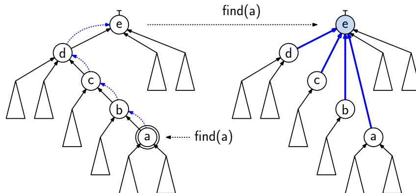
Fig. 117: Find using path compression.
