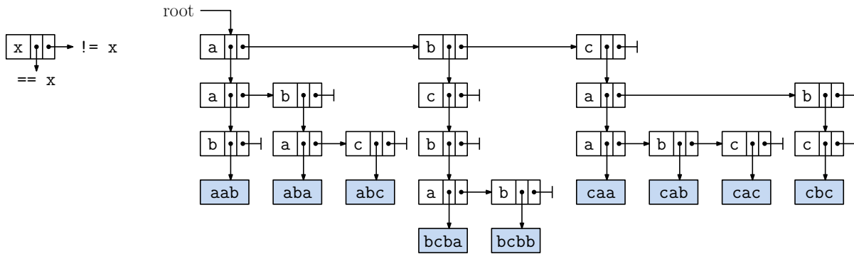
Fig. 101: A de la Briandais tree containing the same strings as in Fig. 99.
