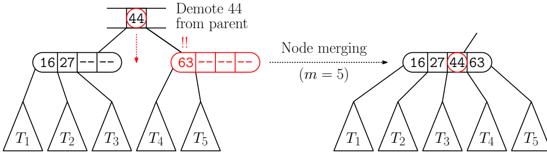
Fig. 62: Node merging for a B-tree of order m = 5 .
