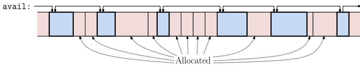
Fig. 107: Dynamic memory allocation block structure.
