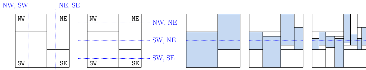
Fig. 82: An axis-parallel line in 2D can stab at most two out of four cells in two levels of the kd-tree decomposition. In general, it stabs 2^i cells at level 2i .
