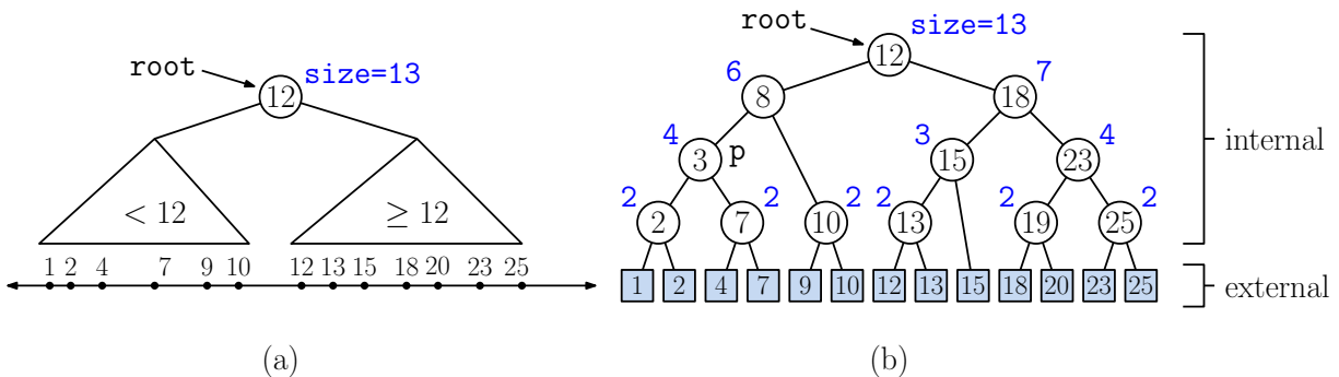
Fig. 94: Extended binary search tree (with sizes).
