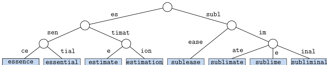
Fig. 104: Alternative (but equivalent) method of drawing the patricia trie of Fig. 103.
