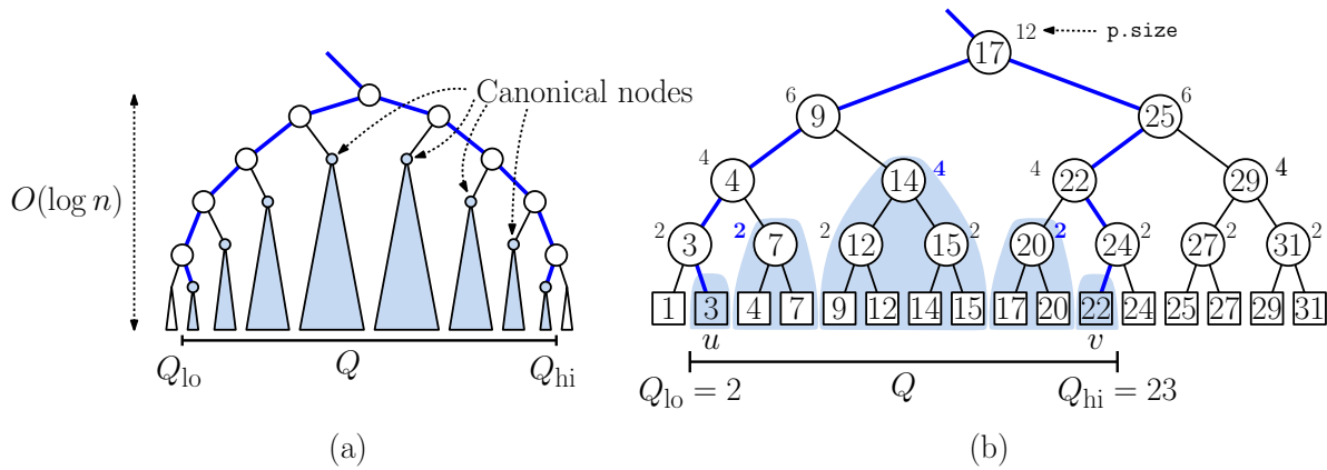
Fig. 96: The canonical subtrees for 1-dimensional range query.
