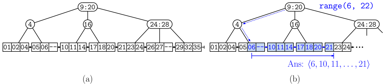
Fig. 66: B+ tree of order m = 3 , where leaves can hold up to 3 keys.
