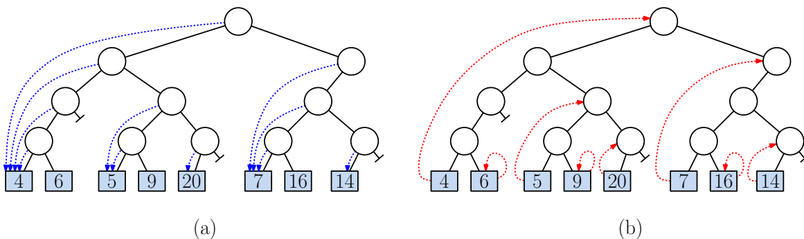
Fig. 124: Enhancements for faster decrease-key() .
