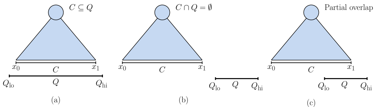
Fig. 97: Range search cases: (a) Q contains p 's cell, (b) Q is disjoint from p 's cell, (c) Q partially overlaps p 's cell.
