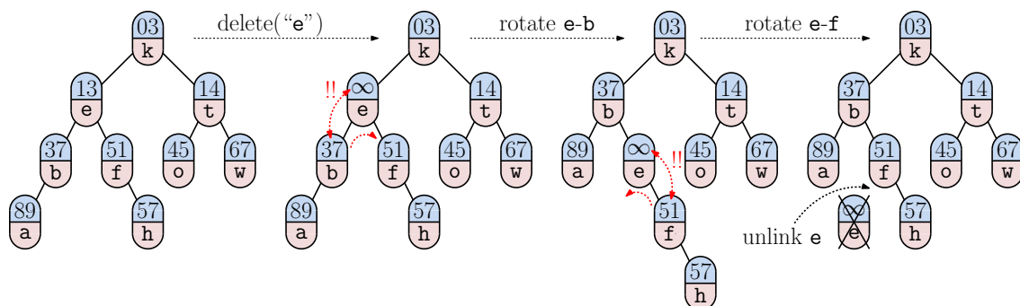
Fig. 44: Treap deletion.
