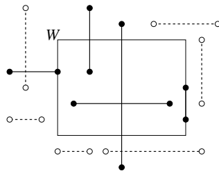
Fig. 132: Window Query.
