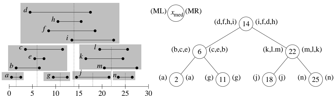
Fig. 134: Interval Tree.
