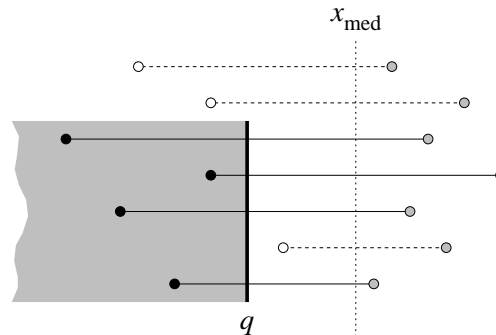
Fig. 135: The segments that stab q lie within the shaded semi-infinite rectangle.
