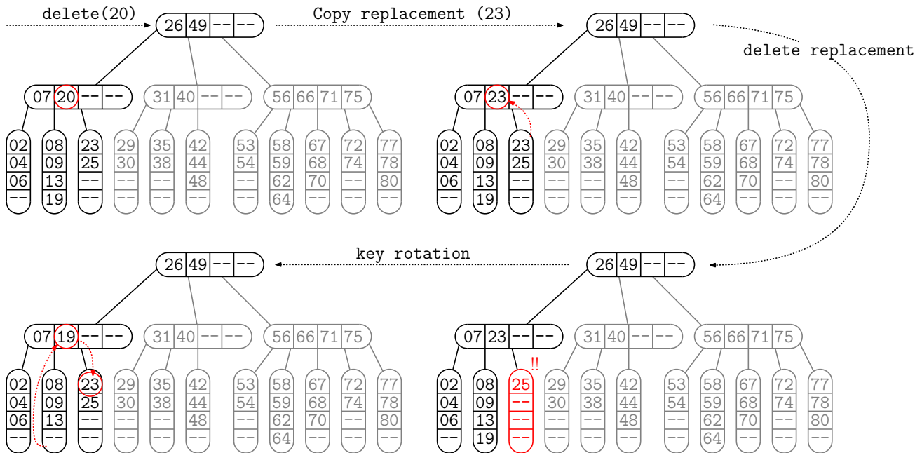
Fig. 64: Deletion of key 20 (order m = 5 ). Since 20 is not a leaf, we find the replacement 23 (inorder successor) and copy it there. We then delete 23 from its leaf, which underflows. The sibling rotates the key 19 to the parent and the parent gives up its key 23.
