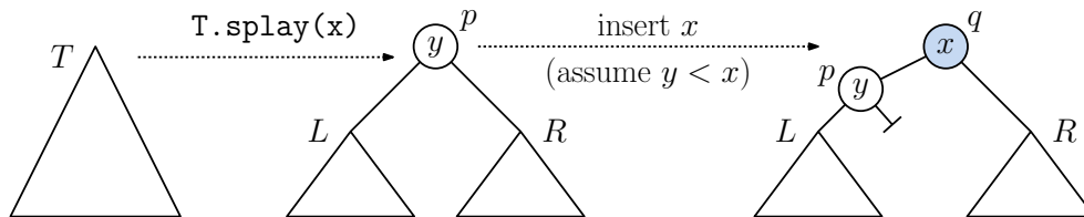
Fig. 56: Splay-tree insertion of x .
