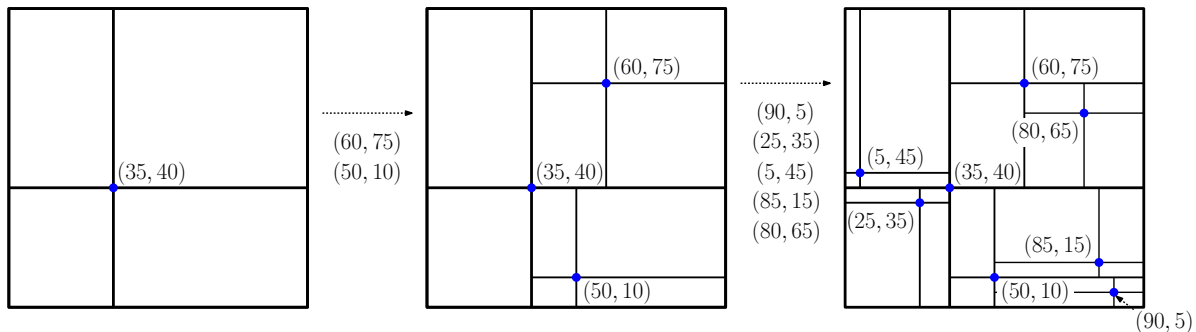
Fig. 70: Point quadtree subdivision.
