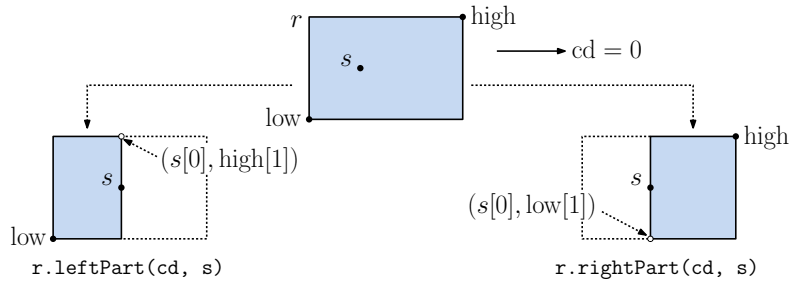
Fig. 79: The functions leftPart and rightPart .
