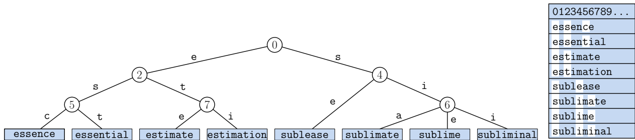
Fig. 103: A patricia trie for a set of strings. Each node is labeled with the index of the character and each edge is labeled with the matching character for this branch.
