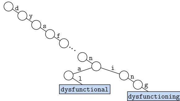
Fig. 102: Space wastage due to long degenerate paths in traditional tries storing “dysfunctional” and “dysfunctioning”.
