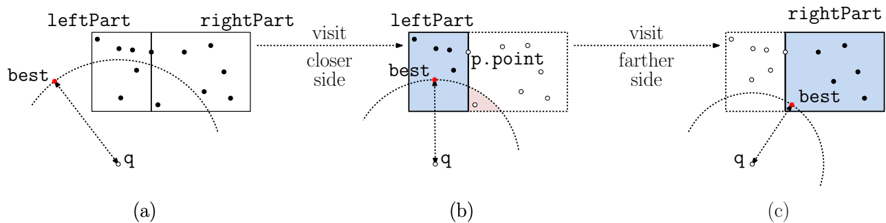
Fig. 85: Nearest-neighbor searching.
