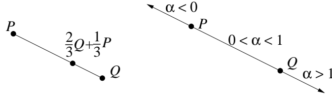
Fig. 130: Affine combinations.
