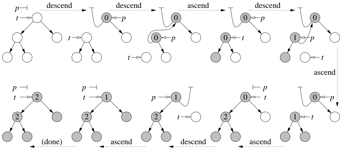
Fig. 137: Marking using link redirection.
