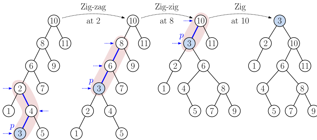
Fig. 6: The full splay operation on p .
