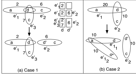
Figure 3: In-graph replication
