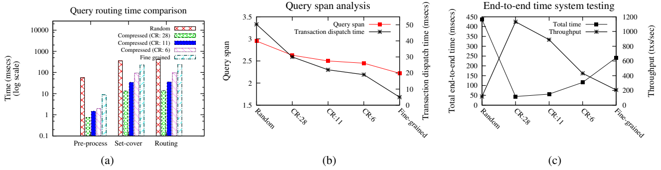
Figure 6: (a) Effect of hypergraph compression in minimizing the query pre-processing time and the set-cover computation time (note that the y -axis is in log scale); (b) The transaction dispatch time is directly dependent on the query span. (c) End-to-end system performance in terms of the end-to-end transaction time and the throughput for the compared schemes.
