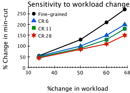
Figure 7: Fine-grained approach is more sensitive to workload changes than the compressed approach
