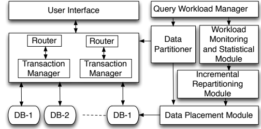
Figure 1: System architecture
