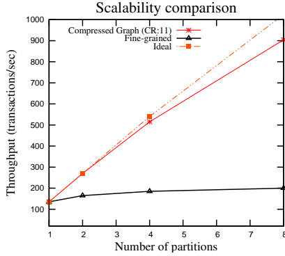
Figure 8: Effect of increasing parallelism on throughput: due to the high query routing costs, the fine-grained approach is not able to effectively utilize the available parallelism.
