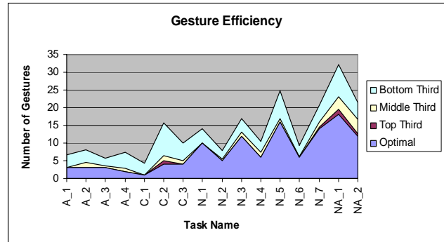
Figure 5. Average number of gestures per task compared with the optimum.
