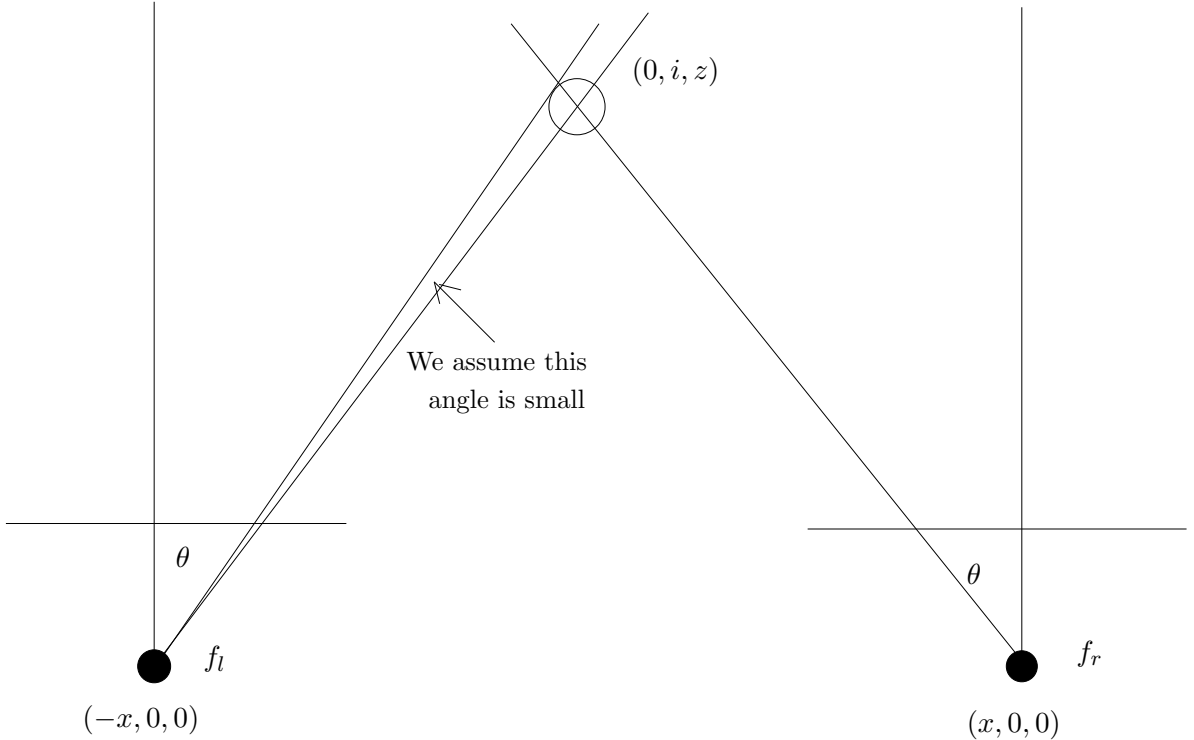
Figure 1: Our very simplified model of faces.
