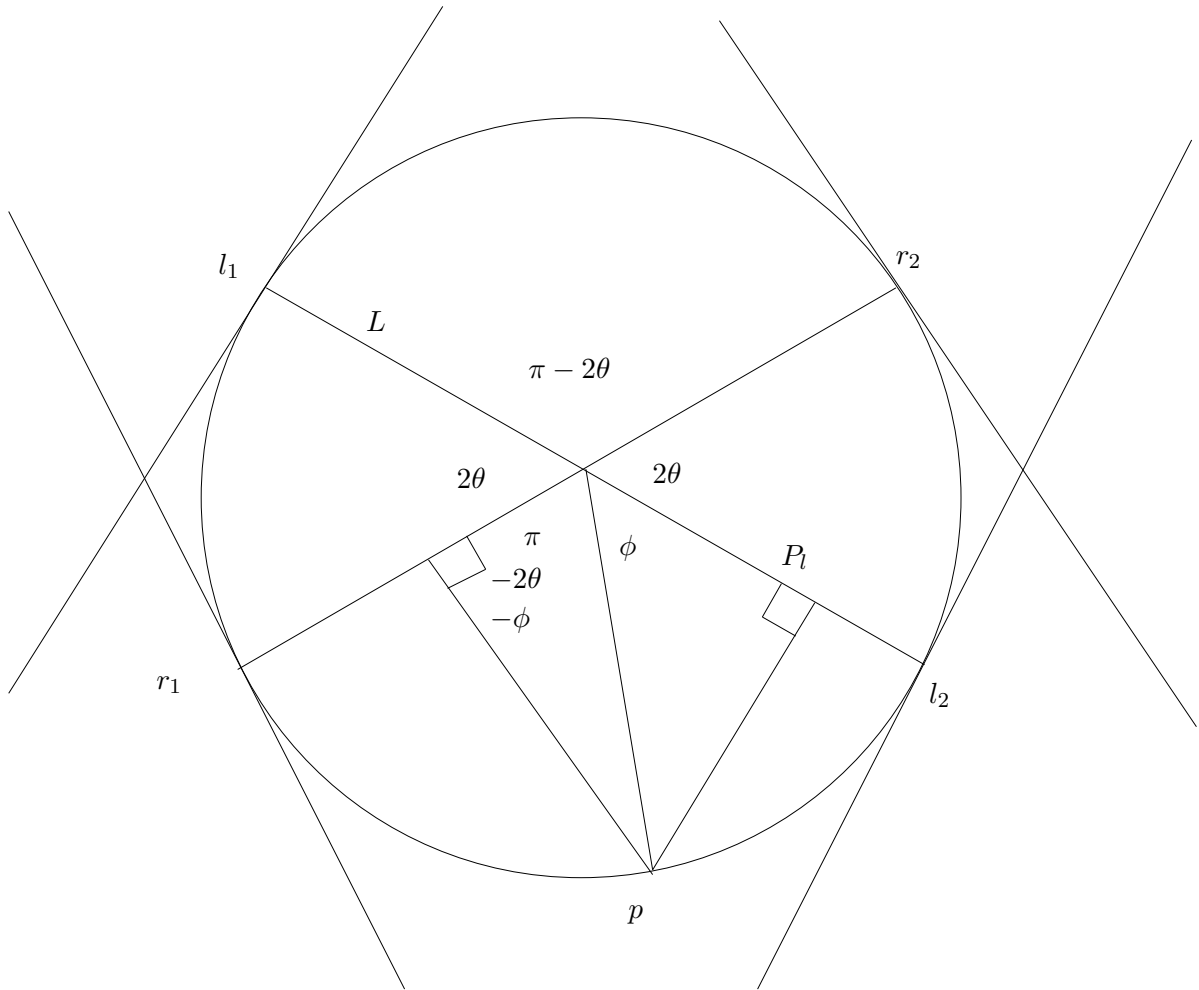
Figure 2: The circle parameterized by the angle \phi .
