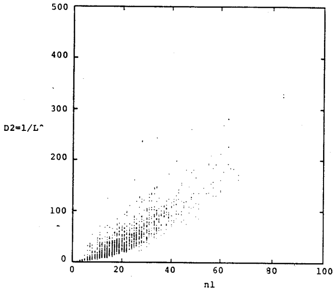
Fig. 5. Difficulty versus unique operator count (1794 modules).
