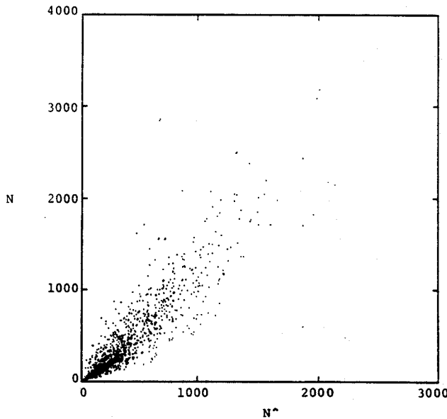
Fig. 1. Observed versus estimated length (1794 modules).
