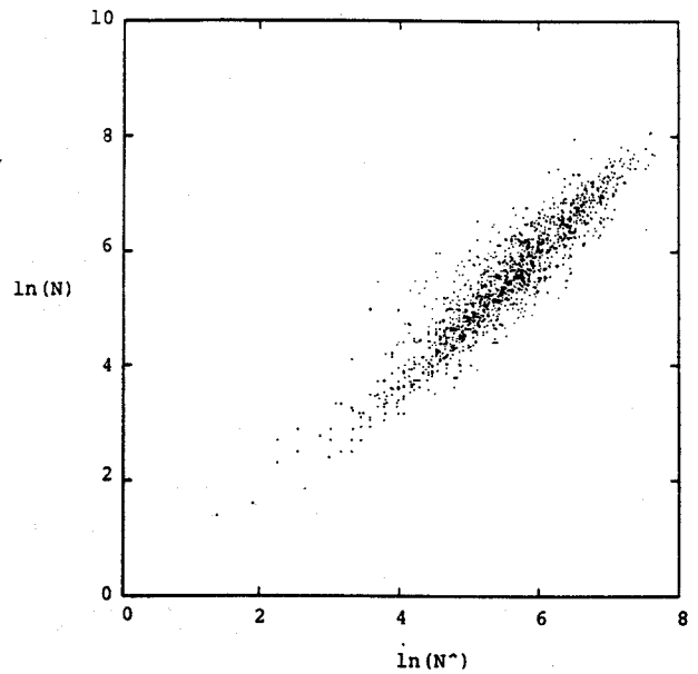
Fig. 2. Log-log plot of observed versus estimated length (1794 modules).
