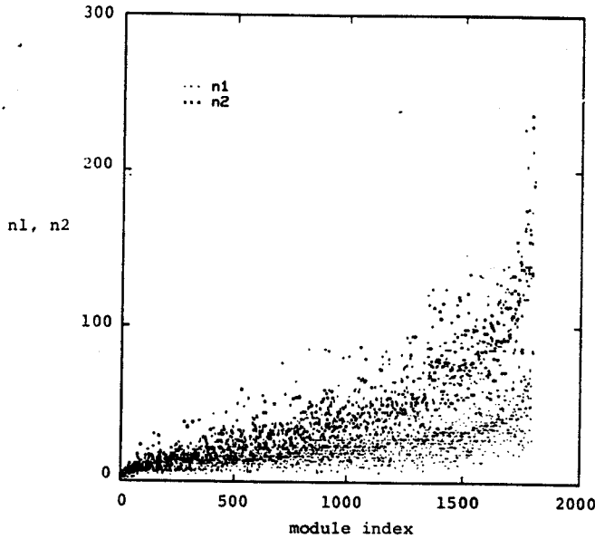
Fig. 4. Unique operators and operands ordered and indexed by length (1794 modules).
