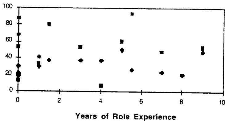
Figure 9b. PBR defect rate versus role experience in the 1995 run.
