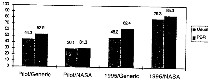
Figure 3. Simulated scores for undiluted teams.
