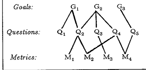
Figure 1. Goal/question/metric paradigm.
