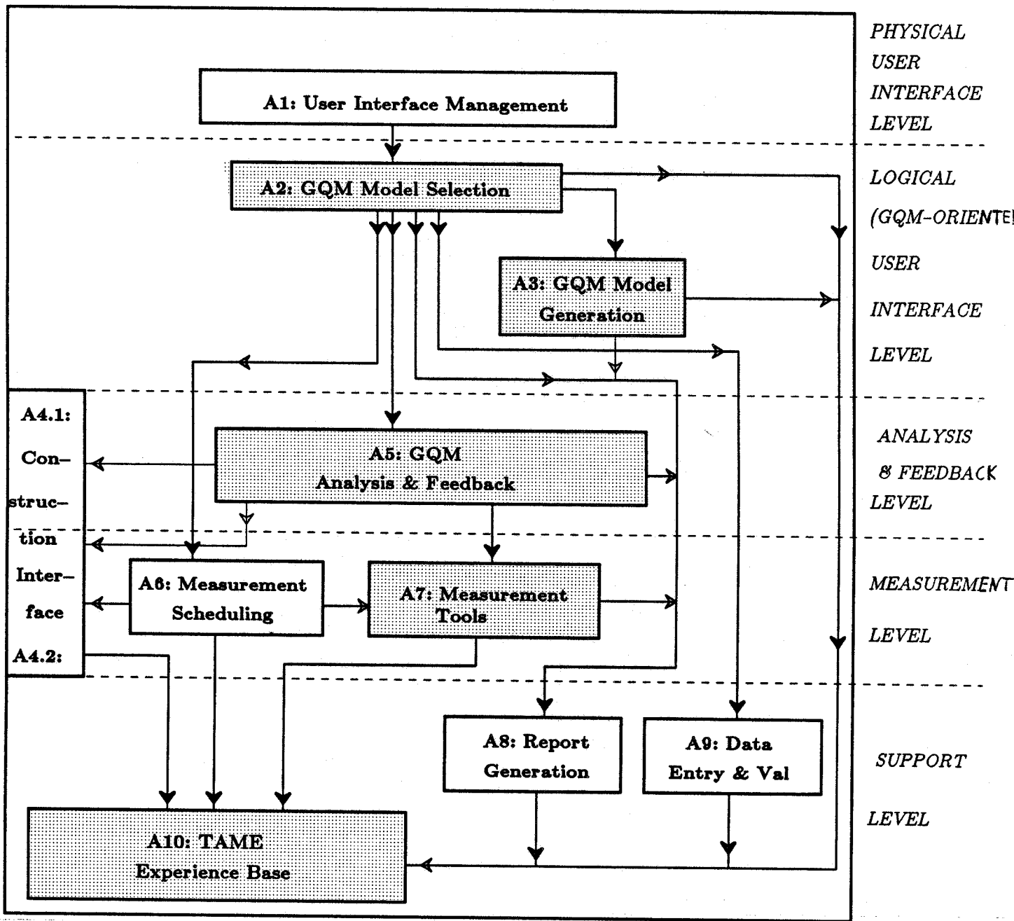
Figure 2: Architectural Design of the TAME System
