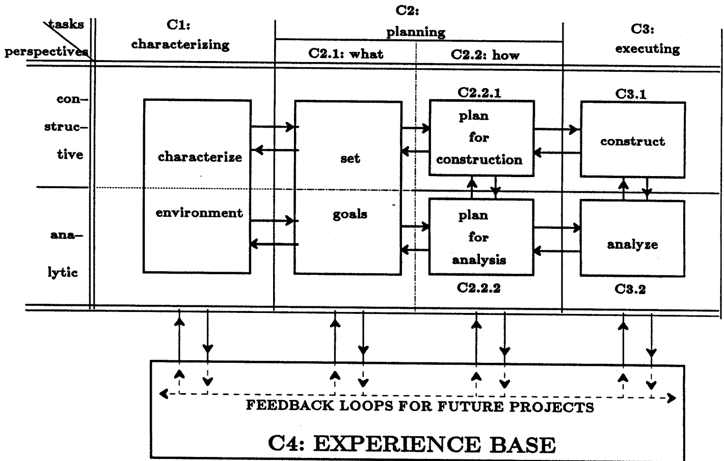
Figure 1: The Improvement-Oriented TAME Software Process Model
