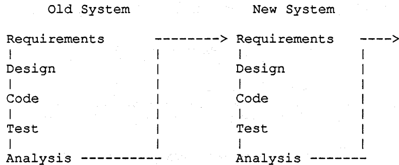
Figure 2. Iterative Enhancement Model
