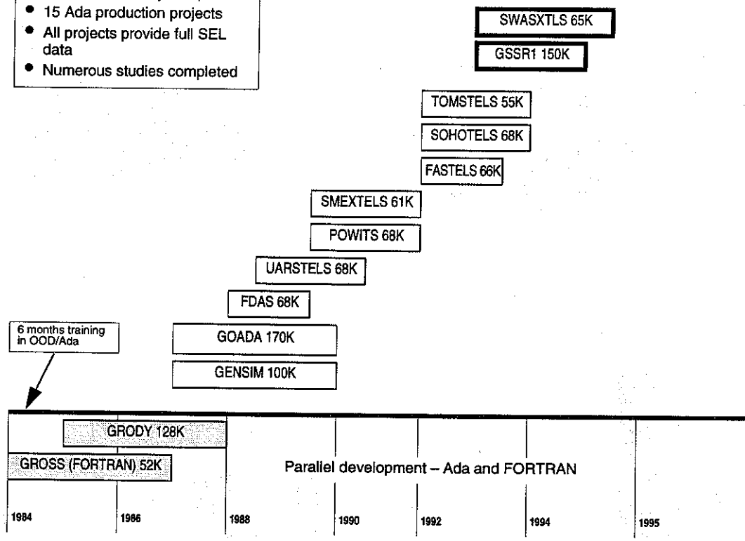
Figure 18: SEL Ada/Object-Oriented Technology (OOT) Projects
