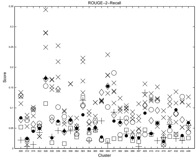
Figure 13. ROUGE-2 recall scores for DUC03 Task 4 data for the human (x) and summarization module (o) summaries, along with the top scoring QCS (•), QL (□), QS (+), and CS (◊) summaries.
