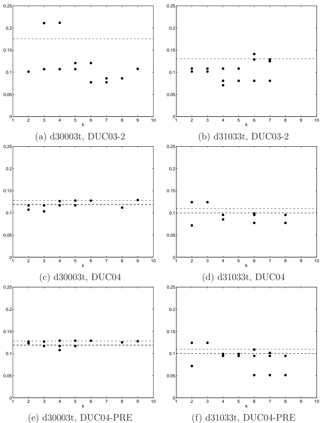
Figure 11. ROUGE-SU4 recall scores for the QCS summaries for clusters d30003t and d31033t as a function of the number of clusters formed ( k ). The dotted lines represent the corresponding scores for the summarization module summaries.
