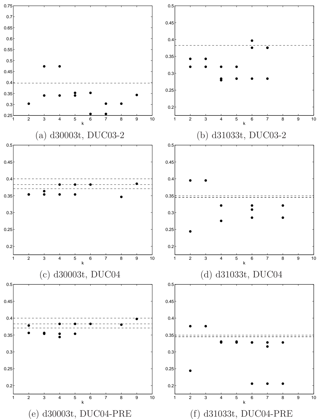
Figure 9. ROUGE-1 recall scores for the QCS summaries for clusters d30003t and d31033t as a function of the number of clusters formed ( k ). The dotted lines represent the corresponding scores for the summarization module summaries.
