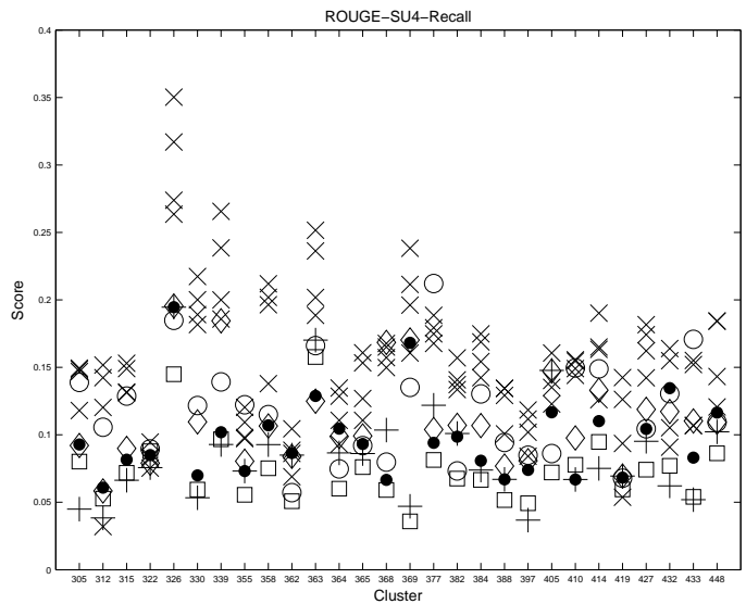
Figure 14. ROUGE-SU4 recall scores for DUC03 Task 4 data for the human (x) and summarization module (o) summaries, along with the top scoring QCS (•), QL (□), QS (+), and CS (◊) summaries.
