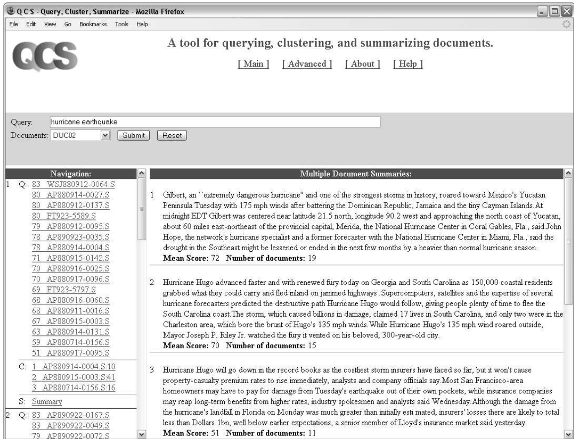
Figure 3. The QCS user interface.
