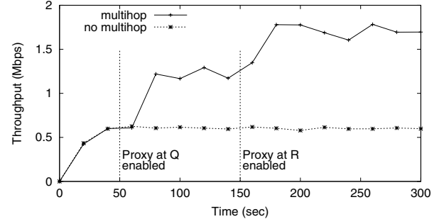
Fig. 8. Adaptation of multi-hop path using the Replacement operation. The sender is at C in Figure 6, and two proxy-enabled clients are at Q and R , respectively. The two upward transitions in bandwidth, corresponds to the adoption of each proxy in the multi-hop path.
