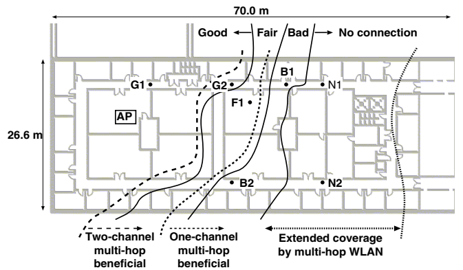
Fig. 2. Potential data throughput improvement by using multi-hop extensions to the currently deployed WLAN in the 4th floor of the A.V. Williams building. The “Good,” “Fair,” “Bad,” and “No Connection” marks the performance of the single-hop WLAN. The multi-hop benefits shown in this figure are obtained using two hop paths.
