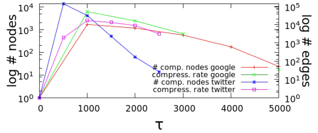
Figure 9: Compression statistics varying \tau .
