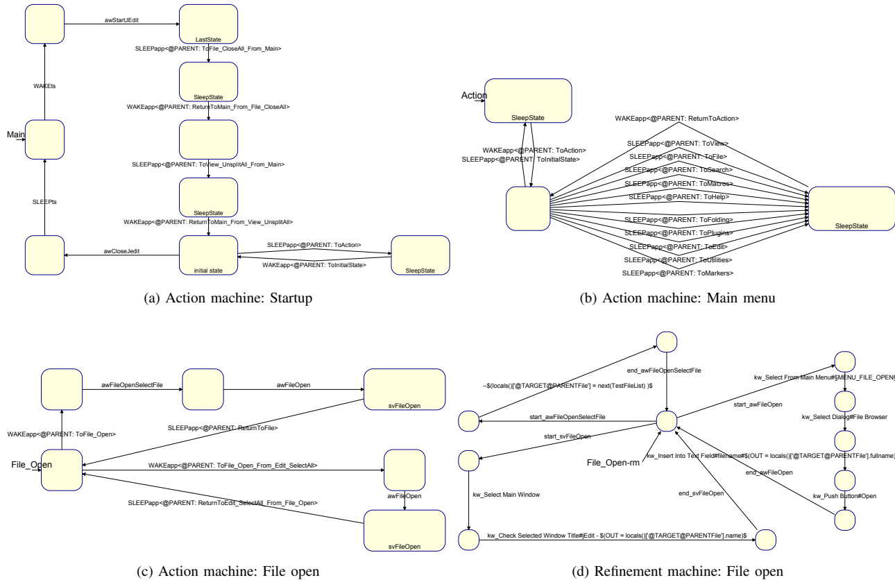
Figure 4: jEdit models
