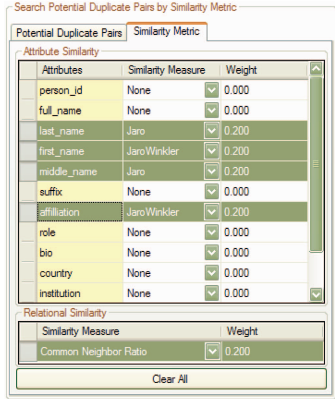
Fig. 2. The similarity metric tab in the potential duplicate viewer allows users to use both attribute and relational similarity measures for computing the similarity between the comparing entities.
