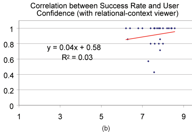
Fig. 10. Correlation between success rate and user confidence. (a) Scatter plot of 48 study tasks with their overall success rate and average user confidence. (b) Scatter plot of 48 study tasks with average success rate and user confidence when the relational context viewer was used.
