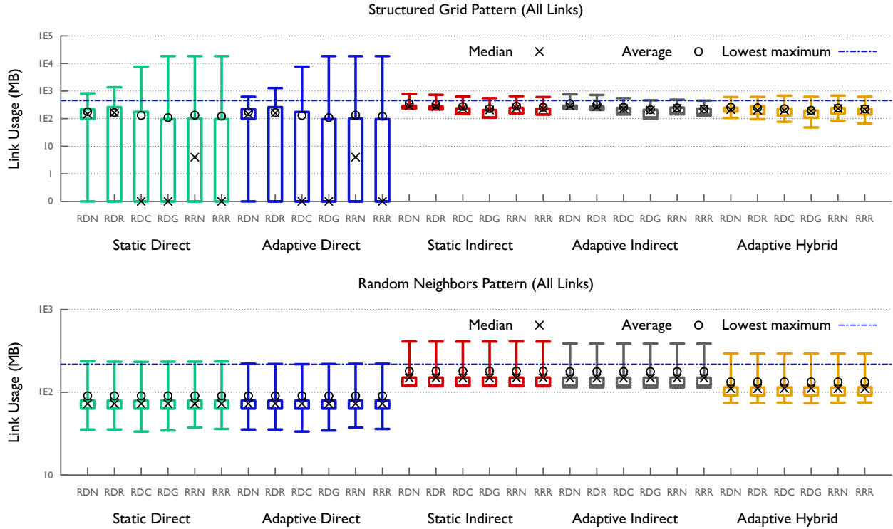
Fig. 5: Structured Grid Pattern (4D Stencil) and Random Neighbors Pattern (Spread)
