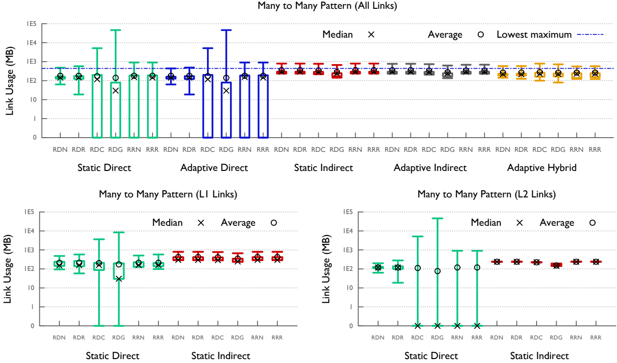
Fig. 7: Many to many pattern (M2M): direct routing with randomized placement has lower average and maximum traffic.
