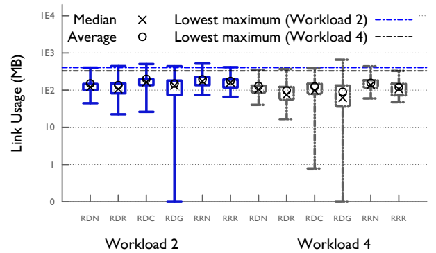
Fig. 10: Job-specific routing traffic distribution (All Links).
