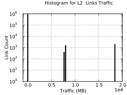
Fig. 6: 4D Stencil: distribution of traffic on L2 links for RDG.
