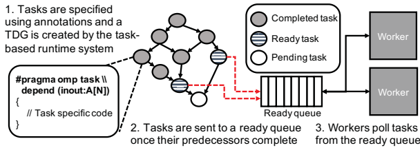
Figure 2. Execution flow in an asynchronous task-based programming model that uses a task dependency graph.
