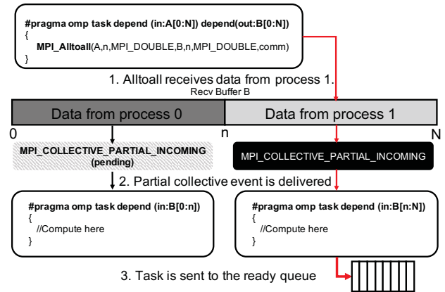
Figure 7. Unlocking of the right task when partial data from process 1 is received leading to a collective callback.
