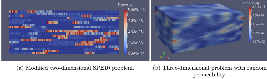
Fig. 4: Heterogeneous Problems.
