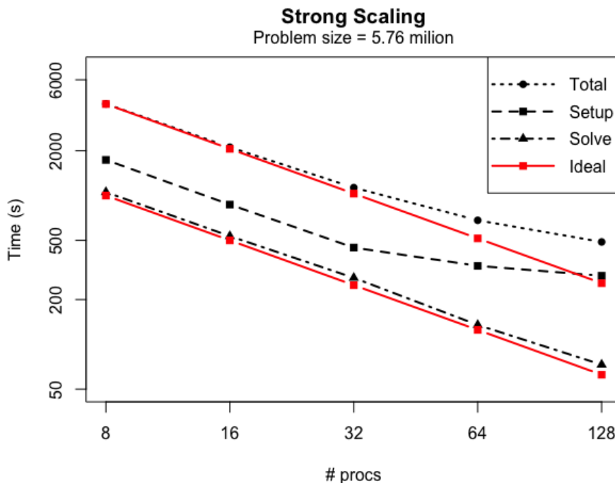
Fig. 5: Strong scaling for the three-dimensional heterogeneous problem. The total runtime for the simulation, the setup, and solve time for the linear solver are reported.
