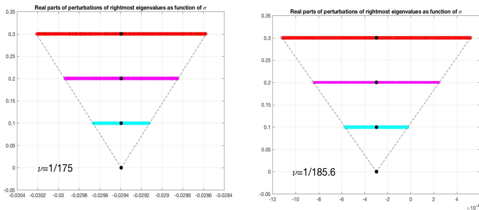
FIG. 3.6. Real parts of surrogate perturbed rightmost eigenvalues for the obstacle problem, for \sigma = .1, .2, \text{ and } .3 , and \nu = 1/175 (left) and \nu = 1/185.6 (right).
