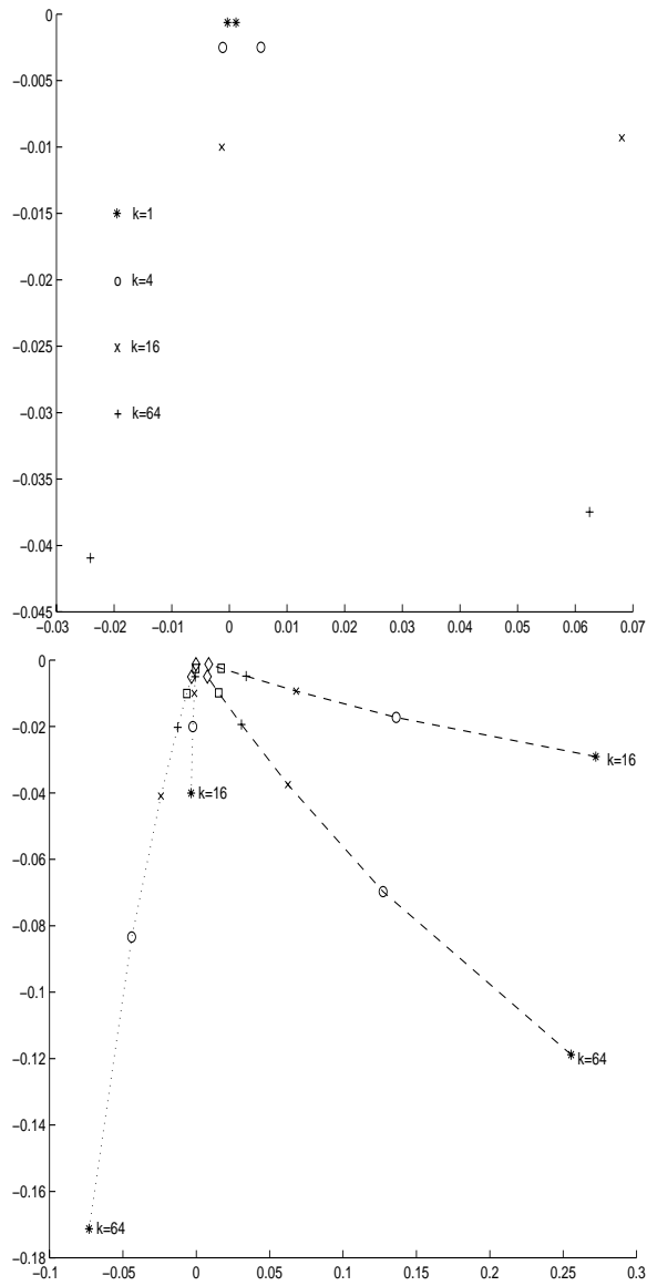
Fig. 2. The two nonunit eigenvalues of the 1-d Sommerfeld problem preconditioned by the 1-d Dirichlet. The top figure shows eigenvalues for values k = 1 (*), k = 4 (o), k = 16 (x) and k = 64 (+) with n = 1600 . The bottom figure shows eigenvalues for values n = 400 (*), n = 800 (o), n = 1600 (x), n = 3200 (+), n = 6400 (□), and n = 12800 (⊙) with k = 16, 64 . For each value of k , the maximal nonunit eigenvalues are connected by a dashed line and the minimal nonunit eigenvalues by a dotted line
