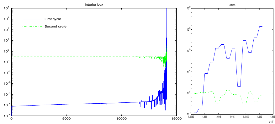
Fig. 11. Polynomial values |p_{40}(\lambda)| for eigenvalues \lambda of Neumann preconditioned operator, k = 30, 60 \times 60 \times 60 grid
