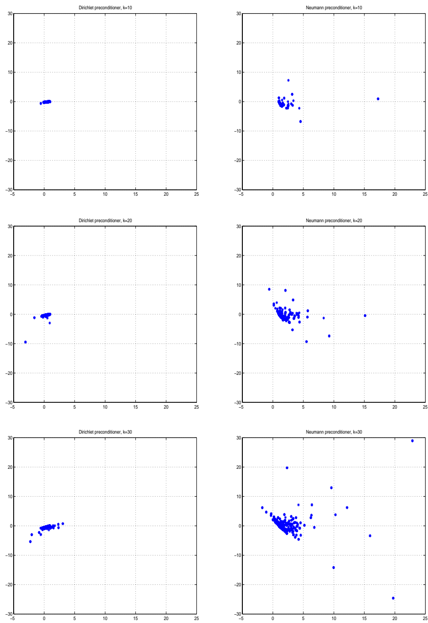
Fig. 7. Eigenvalues of preconditioned three-dimensional problems, for a 60 \times 60 \times 60 grid
