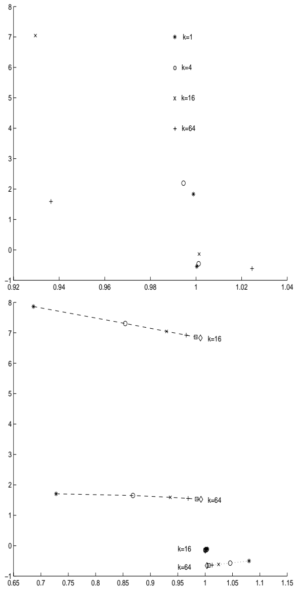
Fig. 1. The two nonunit eigenvalues of the 1-d Sommerfeld problem preconditioned by the 1-d Neumann. The top figure shows eigenvalues for values k = 1 (*), k = 4 ( \circ ), k = 16 ( \times ) and k = 64 (+) with n = 1600 . The bottom figure shows eigenvalues for values n = 400 (*), n = 800 ( \circ ), n = 1600 ( \times ), n = 3200 (+), n = 6400 ( \square ), and n = 12800 ( \diamond ) with k = 16, 64 . For each value of k , the maximal nonunit eigenvalues are connected by a dashed line and the minimal nonunit eigenvalues by a dotted line
