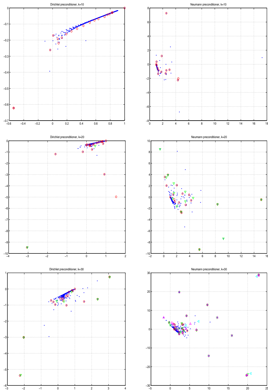
Fig. 8. Eigenvalues ( \cdot ) and generalized Ritz values ( \circ, \nabla, \triangle, \triangleleft, \triangleright, \diamond ) for m = 20 of preconditioned three-dimensional problems, for a 60 \times 60 \times 60 grid
