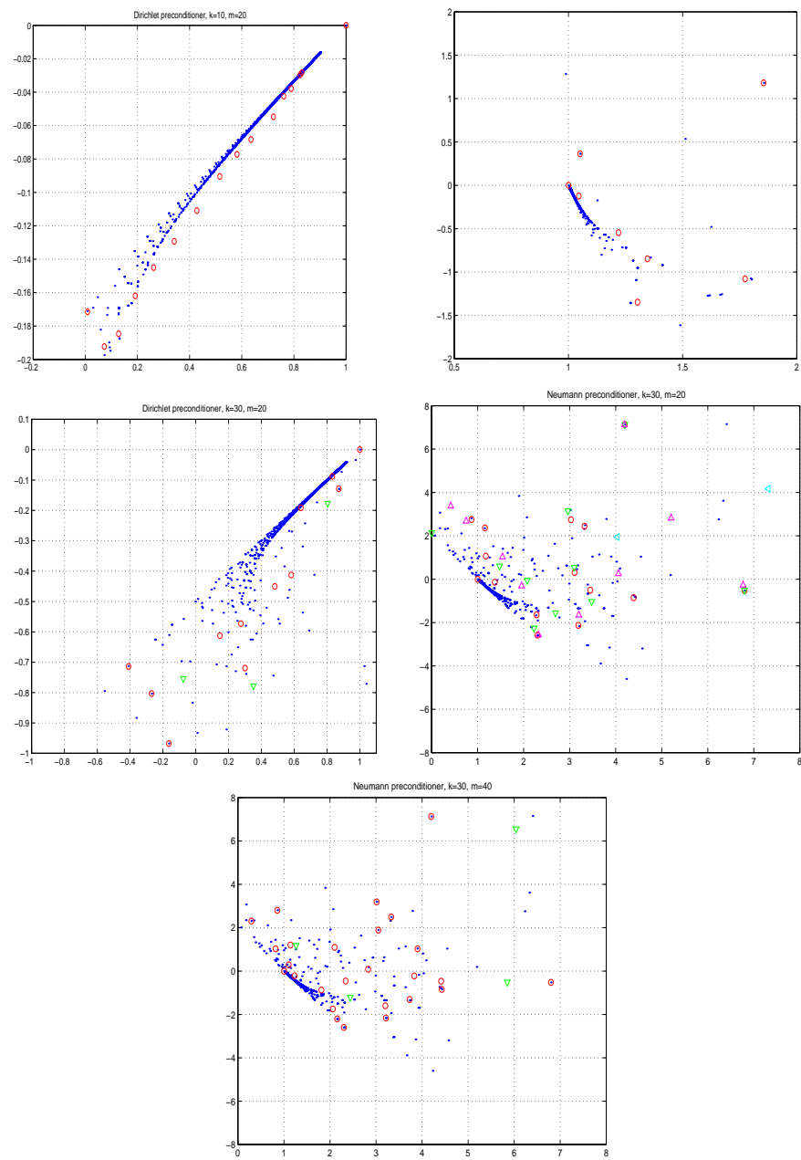
Fig. 9. Subsets of eigenvalues and generalized Ritz values of selected problems, for a 60 \times 60 \times 60 grid
