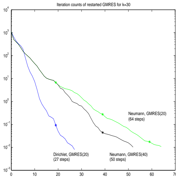
Fig. 13. Iteration counts of preconditioned restarted GMRES for k = 30, 60 \times 60 \times 60 grid
