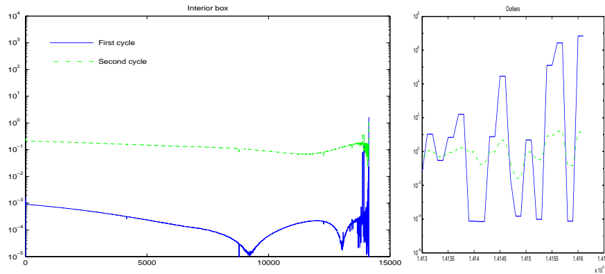
Fig. 12. Polynomial values |p_{20}(\lambda)| for eigenvalues \lambda of Dirichlet preconditioned operator, k = 30, 60 \times 60 \times 60 grid
