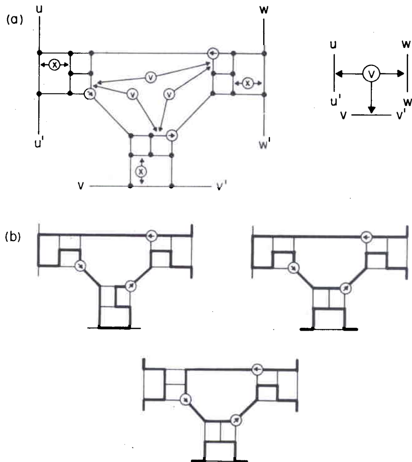
FIG. 6. 3-input or
