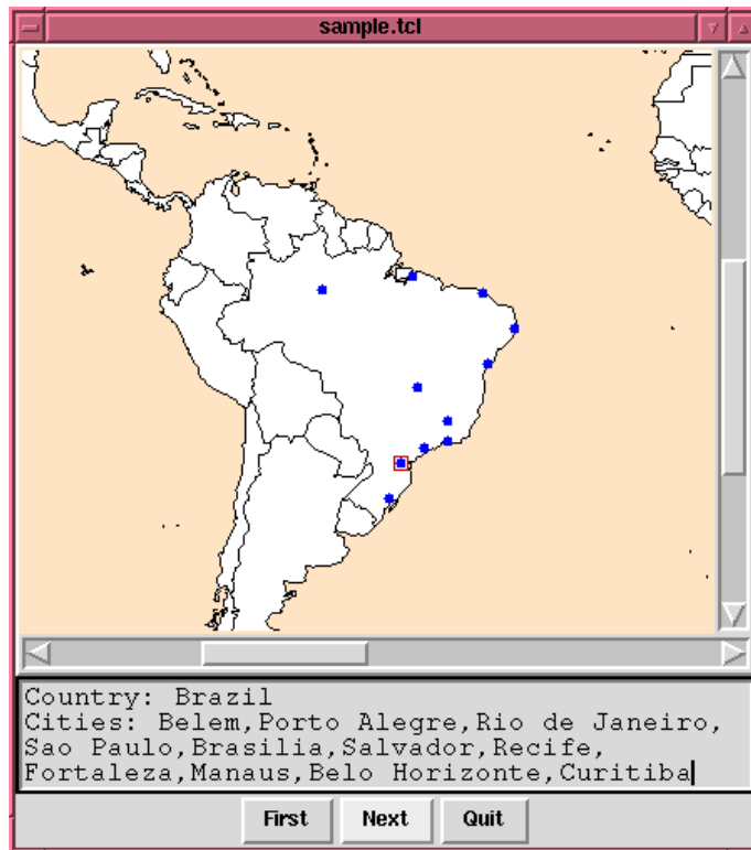
Figure 11: GUI of a sample application for querying cities and countries of the world given in Figure 10.
