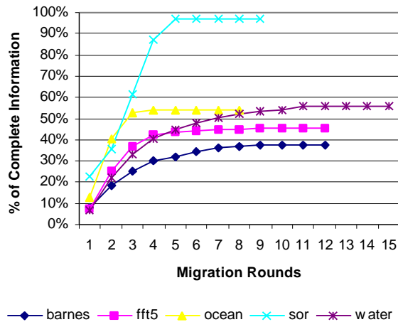
Figure 6: Passive information-gathering
