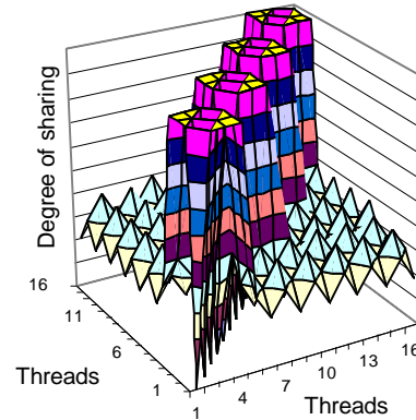
Figure 7: 16-thread FFT
