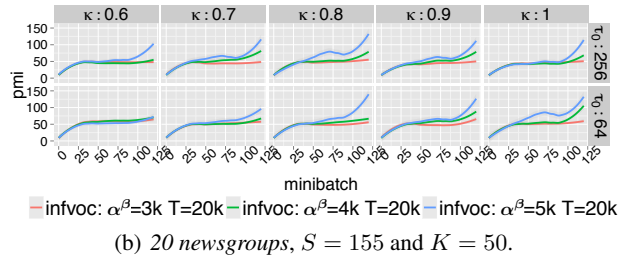
Figure 3. PMI score on two datasets with reordering delay U = 20 against different settings of decay factor \kappa and \tau_0 . A suitable choice of DP scale parameter \alpha^\beta increases the performance significantly. Learning parameters \kappa and \tau_0 jointly define the step decay. Larger step sizes promote better topic evolution.
