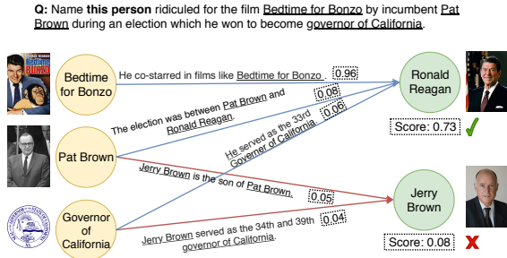
Figure 4: An example DELFT subgraph. The learned edge weights in GNN are in the brackets.
