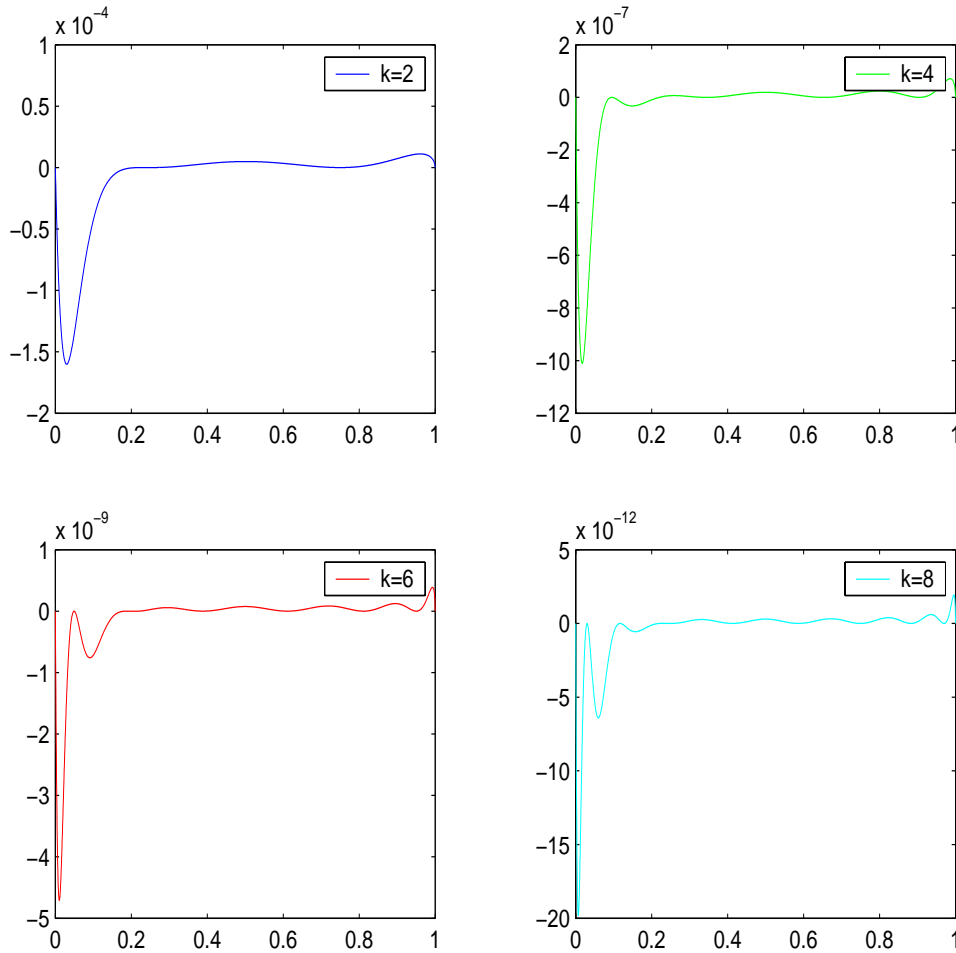
FIG. 3.2. The product p(x)\tilde{p}(x)(w(x) - \tilde{w}(x)) as a function of x for the continuous weight function w(x) = c_0\sqrt{x - x^2} , with perturbation parameter \alpha = 10^{-3} and different number of quadrature nodes k .
