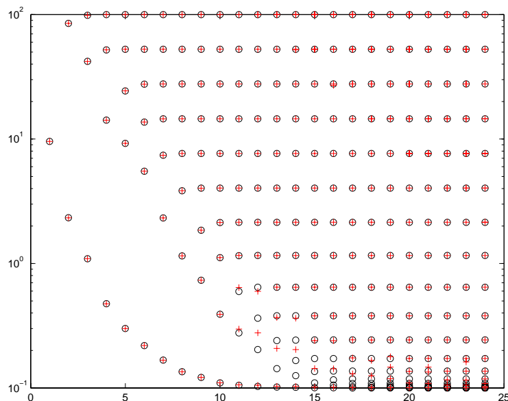
FIG. 4.4. Quadrature nodes corresponding to the distribution function \omega (circles) and \bar{\omega} (plusses). The horizontal axis is the number of nodes k in the quadrature.
