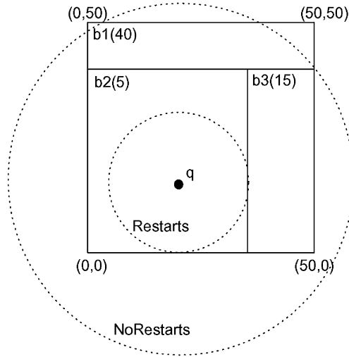
Fig. 7. An Example of Restarts and NoRestarts Strategies in Filter-Restart Approach [Bruno et al. 2002]
