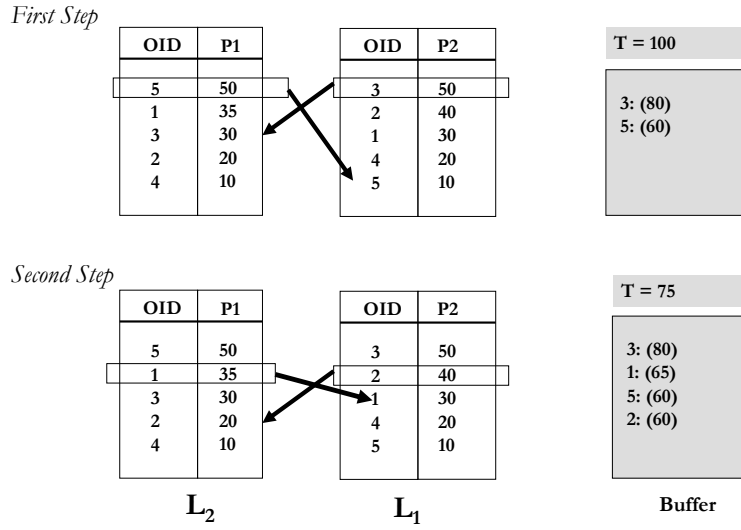
Fig. 5. The Threshold Algorithm (TA)
