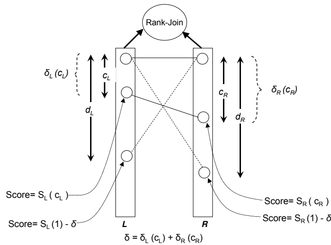
Fig. 18. Estimating Depth of Rank-Join Inputs
