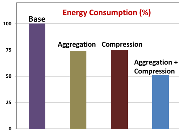
Figure 2: Energy savings with Stratus for web browsing workloads.
