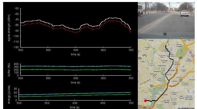
Figure 3: Screenshot of the trace-driven animation showing scheduling in action during a drive.
