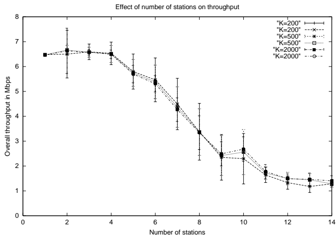
Fig. 1. Throughput with increasing number of stations
