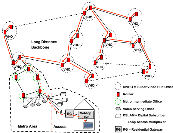
Figure 1. Simplified network architecture
