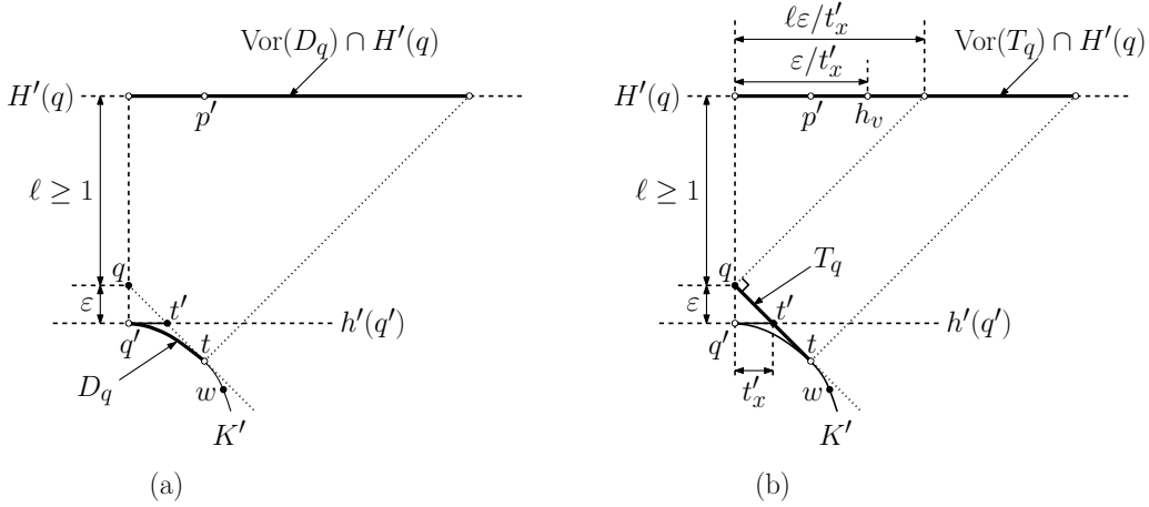
Figure 4: Proof of Lemma 3.2.
