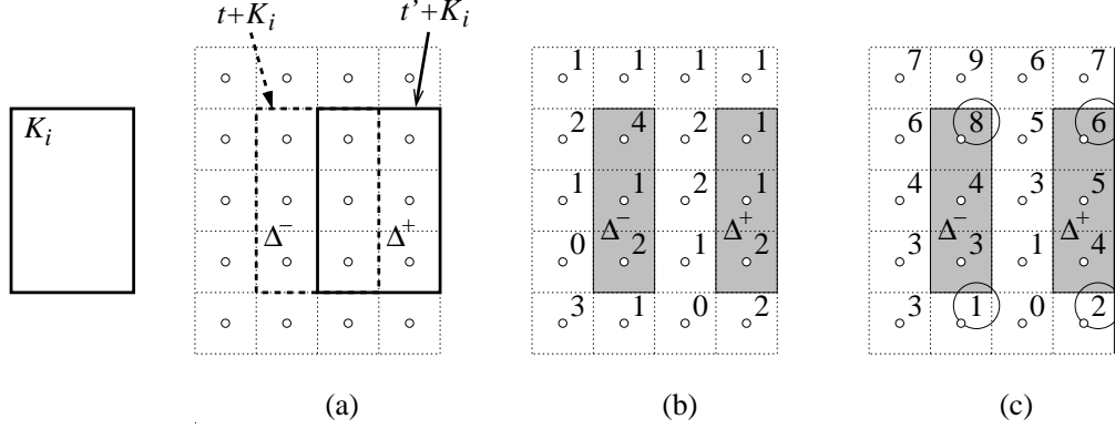
Figure 8: (a) The two translates t + K_i (dotted) and t' + K_i (solid) which form the symmetric difference, (b) the initial image pixel weights, and (c) the weights after computing prefix sums within each column.
