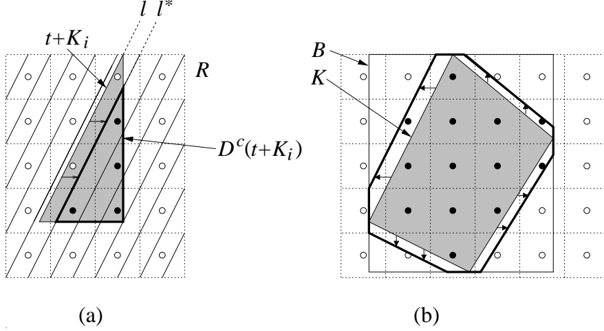
Figure 6: Canonical digitization.
