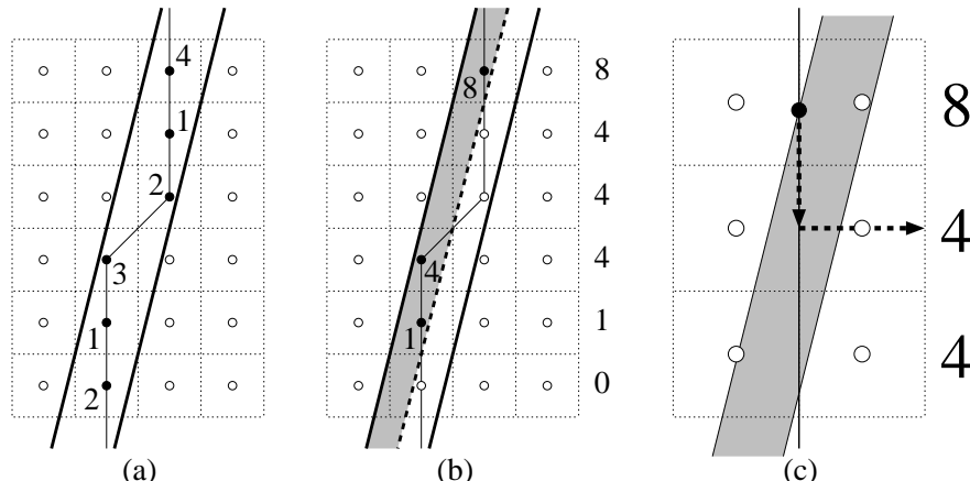
Figure 11: Technical issues in the algorithm.
