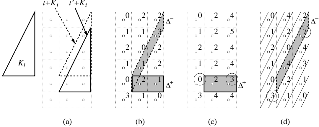
Figure 10: Updating weights for the vertical translation of a triangle.
