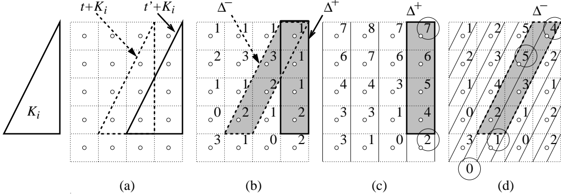
Figure 9: Updating weights for the horizontal translation of a triangle.
