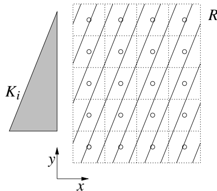
Figure 4: Canonical lines.
