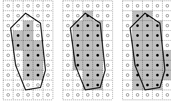
Figure 1: Valid digitizations.
