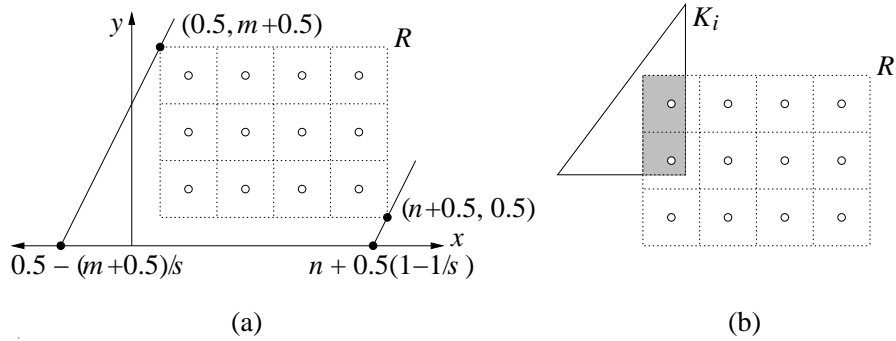
Figure 5: (a) The range of canonical lines and (b) the intersection of a triangle K_i with R .
