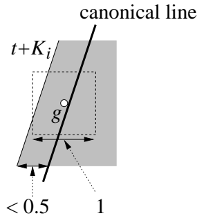
Figure 7: Proof of Lemma 3.
