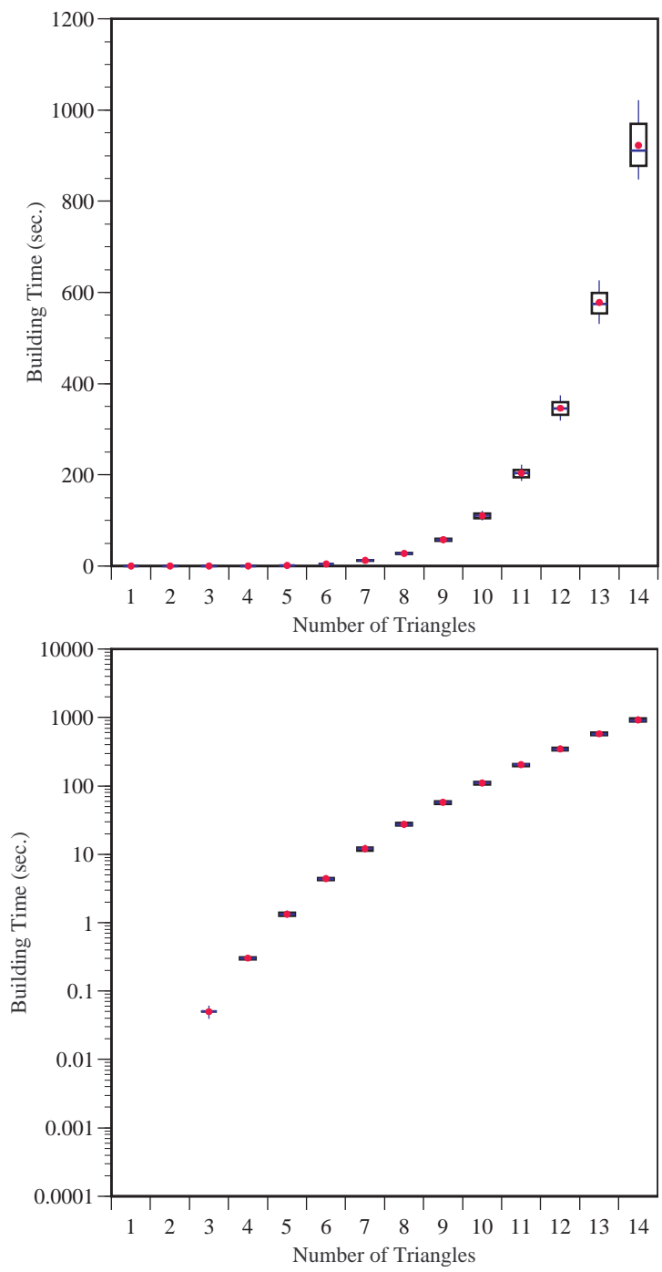
Fig. 9. Building time of Plücker space partition tree.
