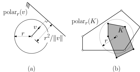
Figure 2: The generalized polar transform.
