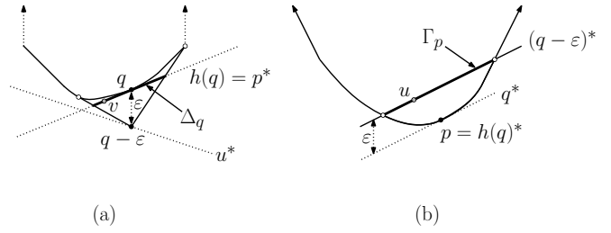
Figure 6: Proof of Lemma 4.1.
