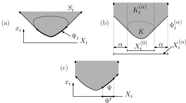
Figure 1: Support sets and projections.
