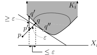
Figure 4: Proof of Lemma 2.2.
