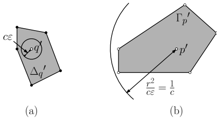
Figure 7: Proof of Lemma 4.2.
