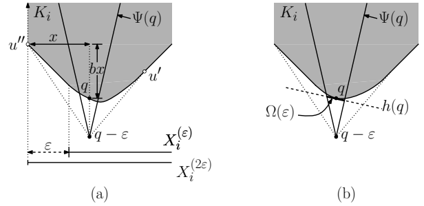
Figure 8: Proof of Lemma 4.2 (continued).
