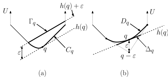
Figure 3: Caps and dual caps.
