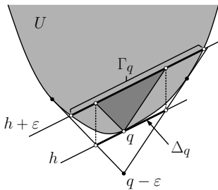
Figure 5: Proof of Lemma 3.1.
