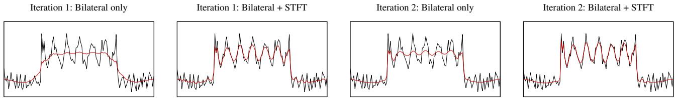
Fig. 2: Intermediate steps of first two iterations of denoising. The bilateral filter and STFT shrinkage cooperate in alternation to denoise the signal. Denoised results in red are compared against the initial noisy signal in black.
