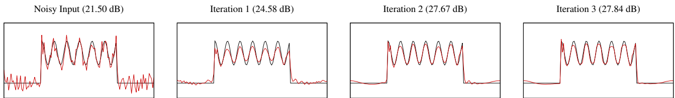
Fig. 3: Progression of denoising. The guide signal in red improves every iteration, approximating the original signal in black.
